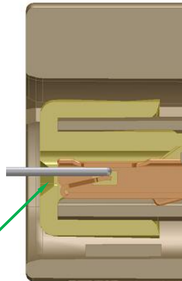
View of probe pin female terminal
