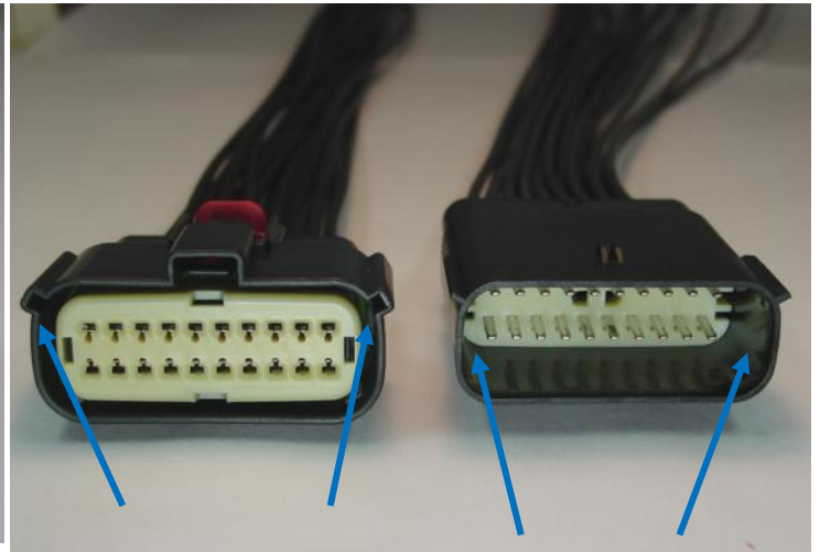
Keying Features
