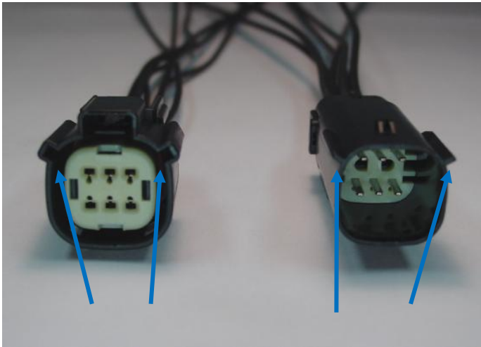
Keying features
