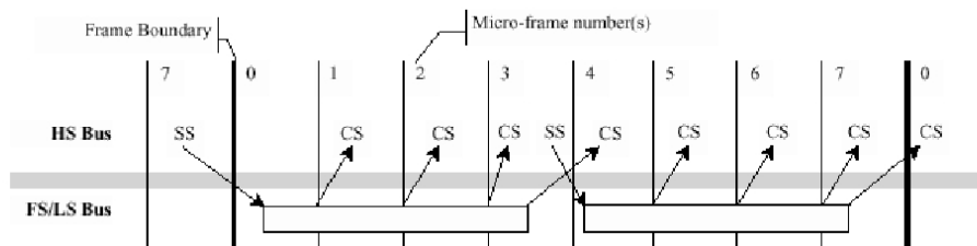
Figure 43-147. Frame Boundary Relationship between HS bus and FS/LS Bus
