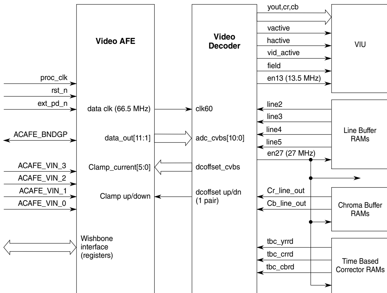
Figure 61-1. Video subsystem block diagram
