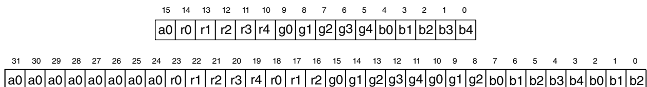
Figure 66-3. ARGB1555 to ARGB8888 Conversion
