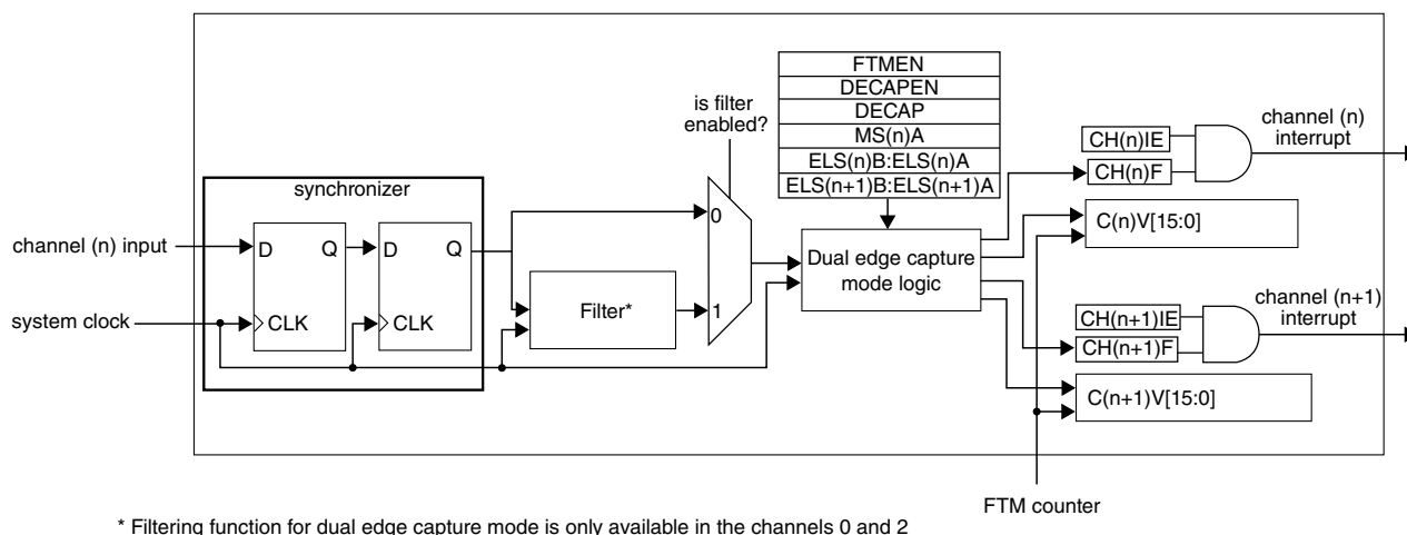
Figure 39-285. Dual Edge Capture mode block diagram
