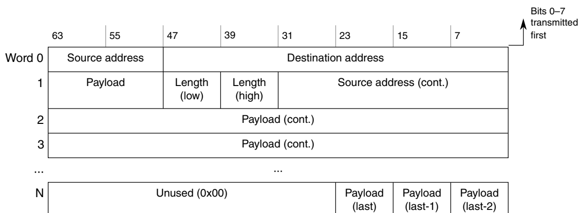
Figure 42-314. Normal Ethernet frame 64-bit mapping example
