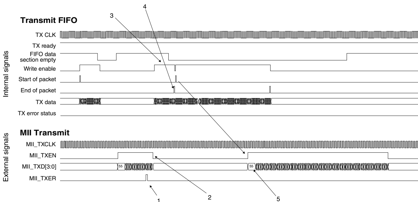
Figure 42-316. Transmit FIFO underflow protection
