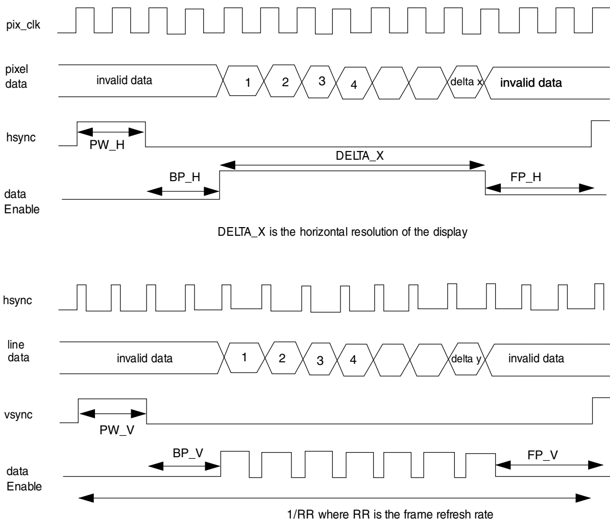
Figure 55-1922. HSYNC and VSYNC timing diagram
