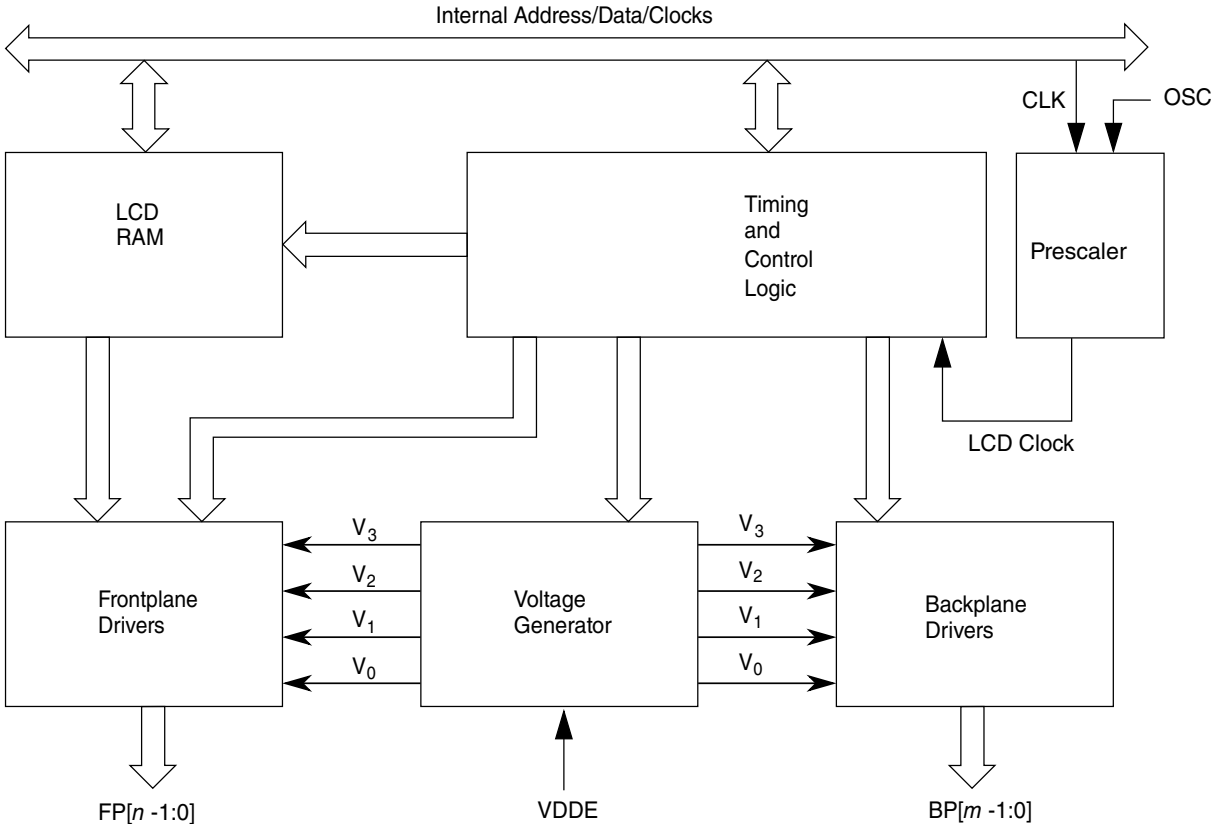
Figure 56-1. Block Diagram
