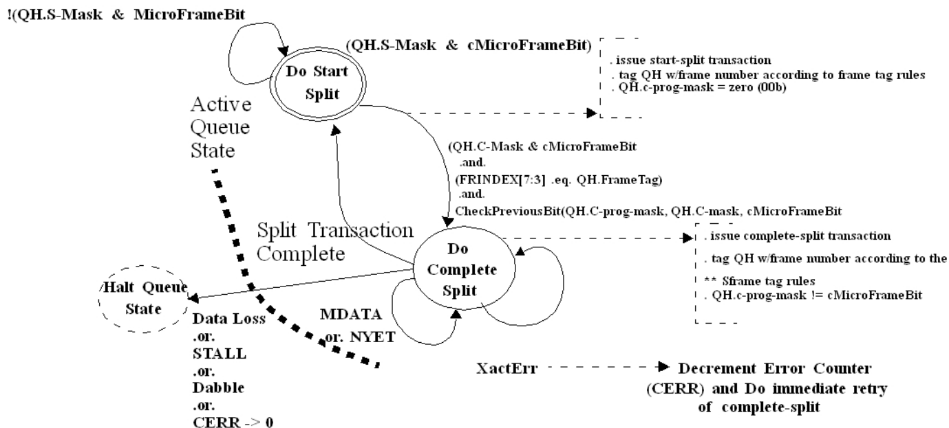
Figure 43-161. Split Transaction State Machine for Interrupt
