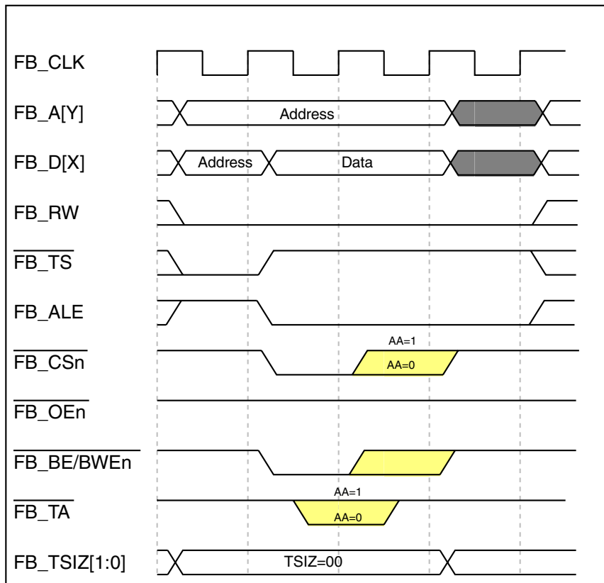
Figure 32-31. Longword-Write Transfer
