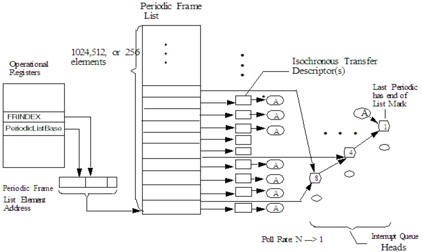
Figure 43-140. Periodic schedule organization
