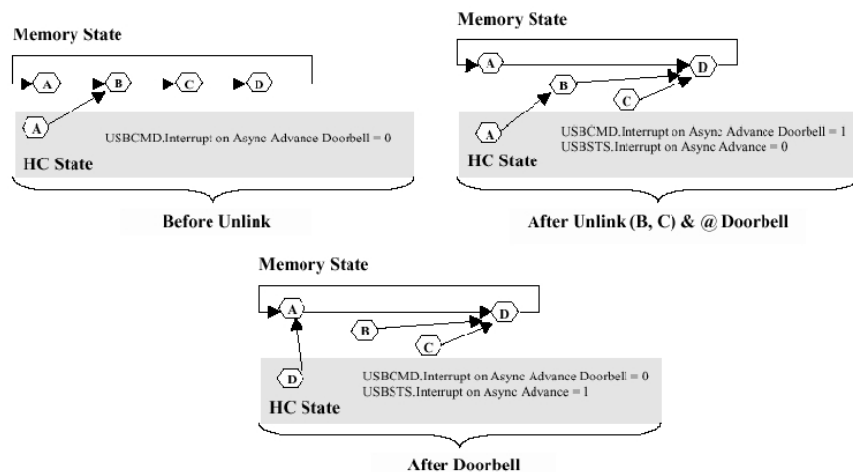
Figure 43-151. Generic Queue Head Unlink Scenario
