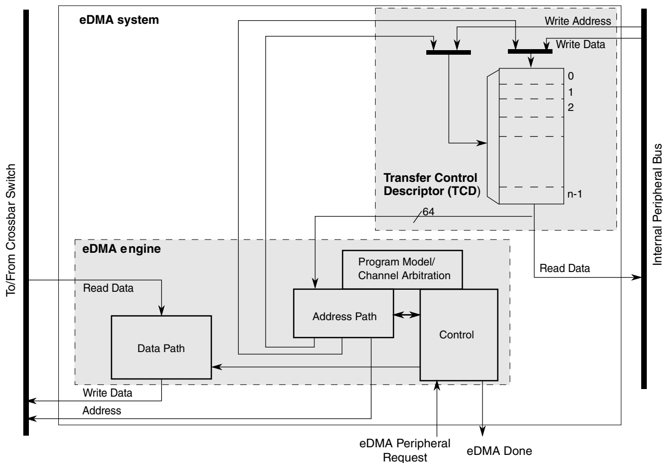
Figure 21-1. eDMA system block diagram
