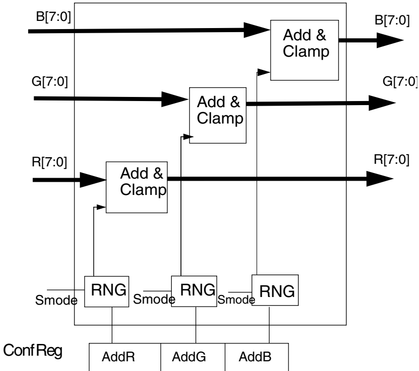
Figure 55-1943. Dithering block diagram
