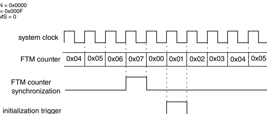
Figure 39-282. Initialization trigger is generated when there is the FTM counter synchronization
