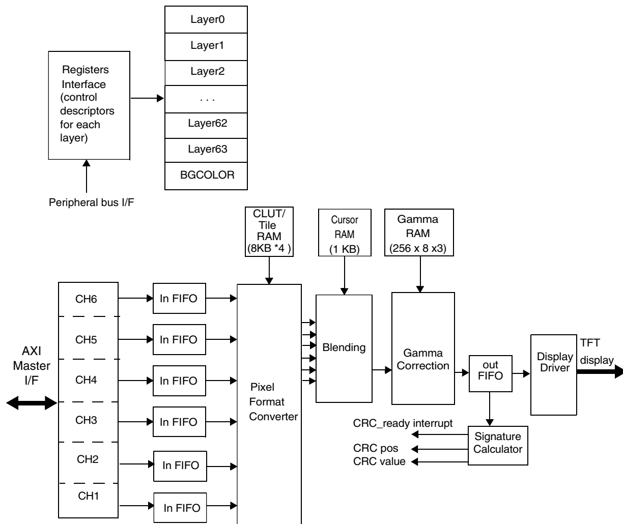
Figure 55-1. Display control unit block diagram
