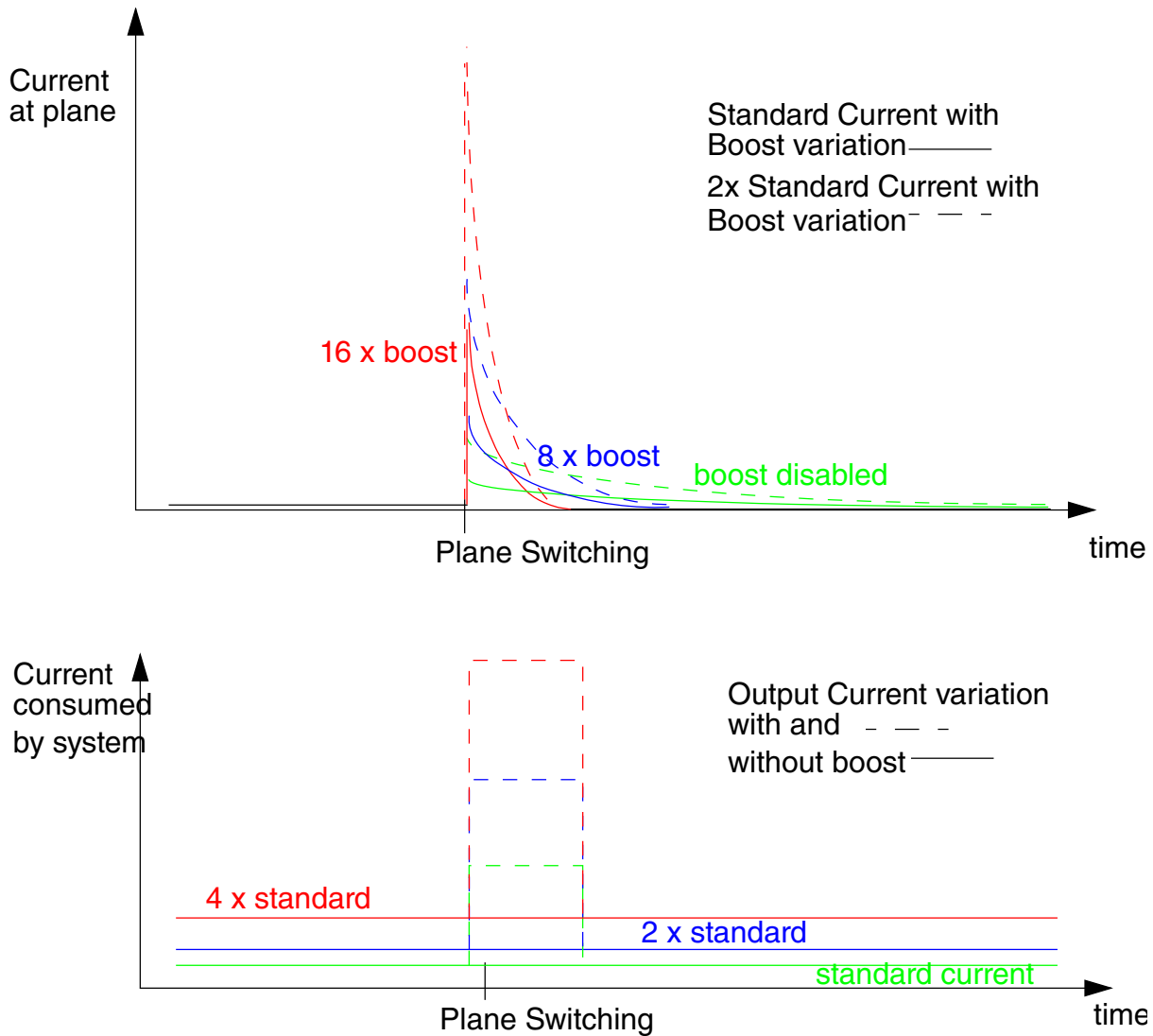
Figure 56-18. PWR, BST, BSTEN Example Diagram
