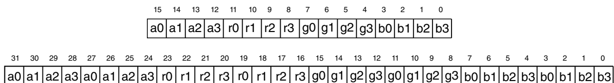
Figure 66-4. ARGB4444 to ARGB8888 Conversion
