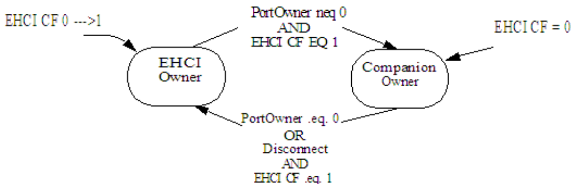
Figure 43-143. Port Owner Handoff State Machine
