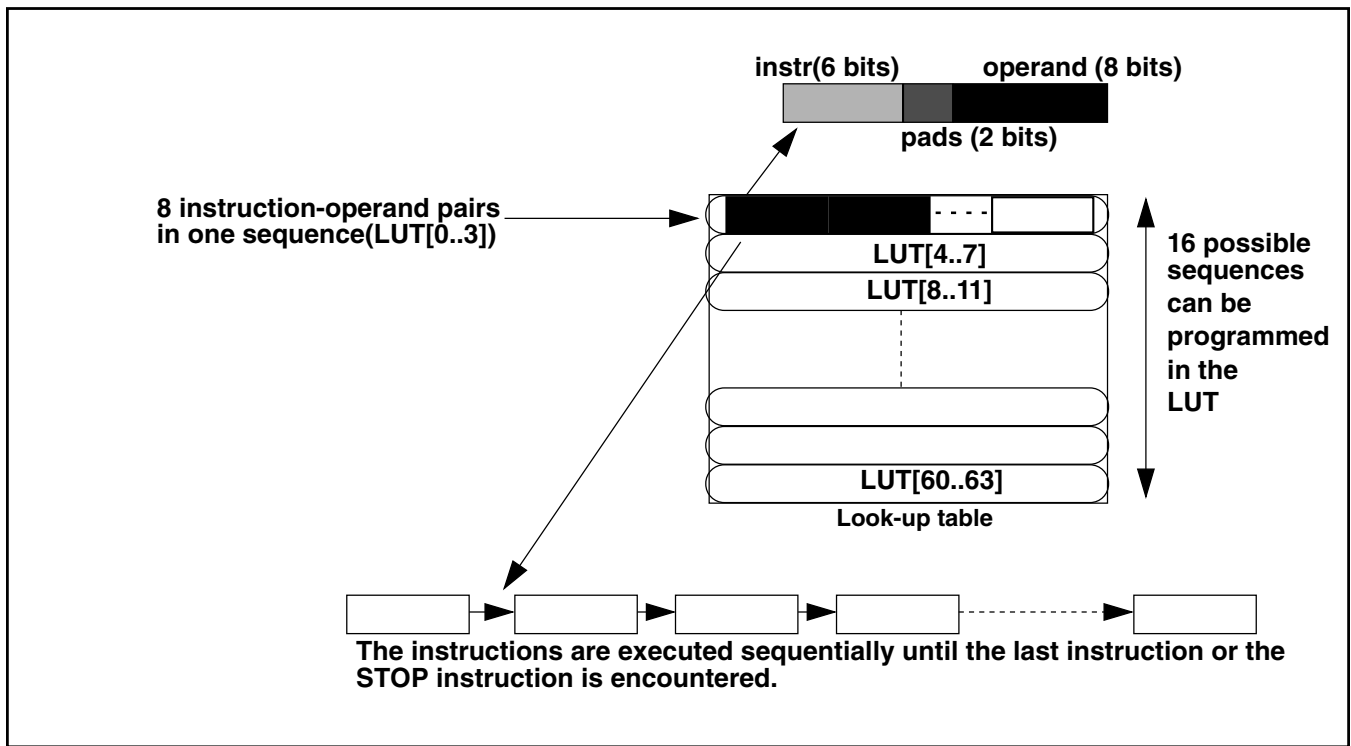
Figure 30-415. LUT and sequence structure
