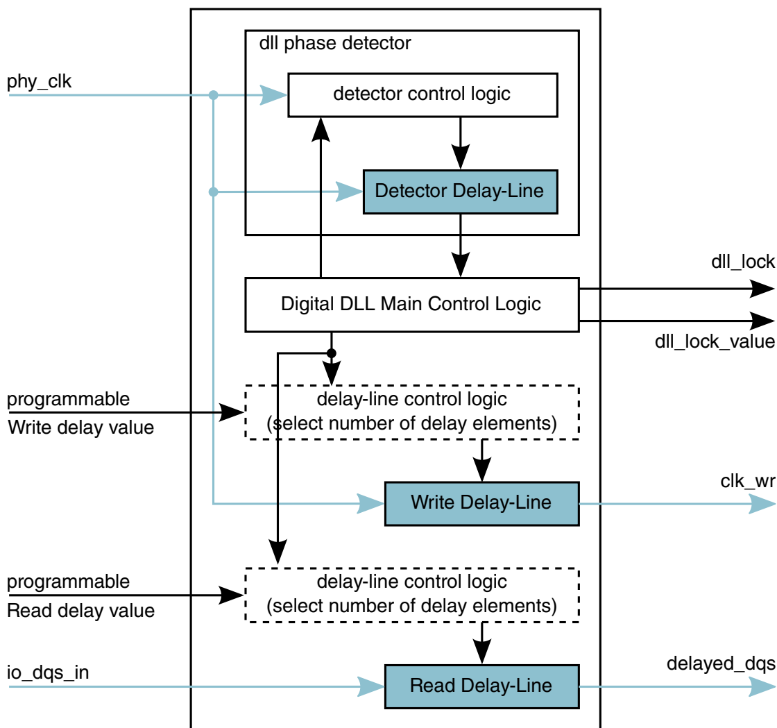
Figure 34-203. Digital DLL
