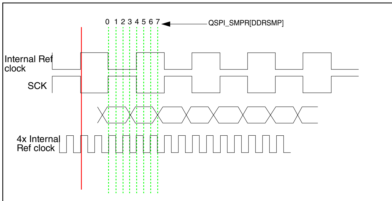
Figure 30-422. DDR sampling edges
