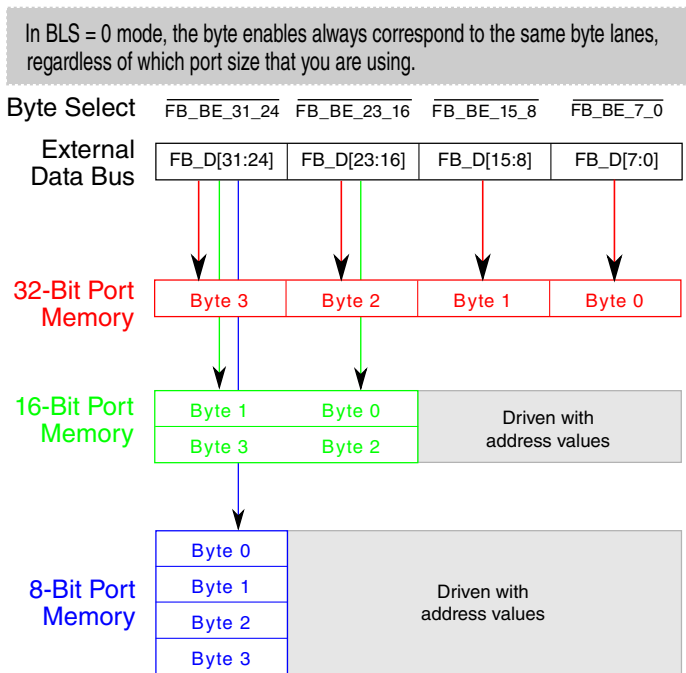
Figure 32-20. Connections for external memory port sizes (CSCRn[BLS] = 0)
