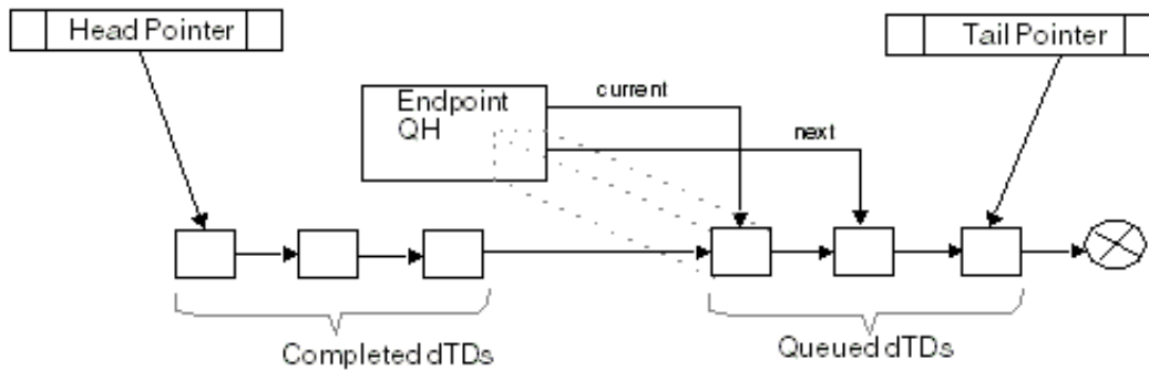
Figure 43-168. Software Link Pointers
