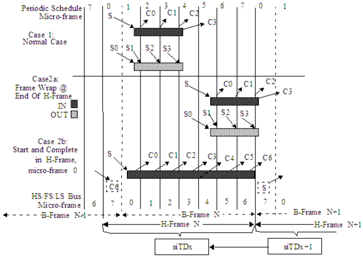
Figure 43-162. Split Transaction, Isochronous Scheduling Boundary Conditions
