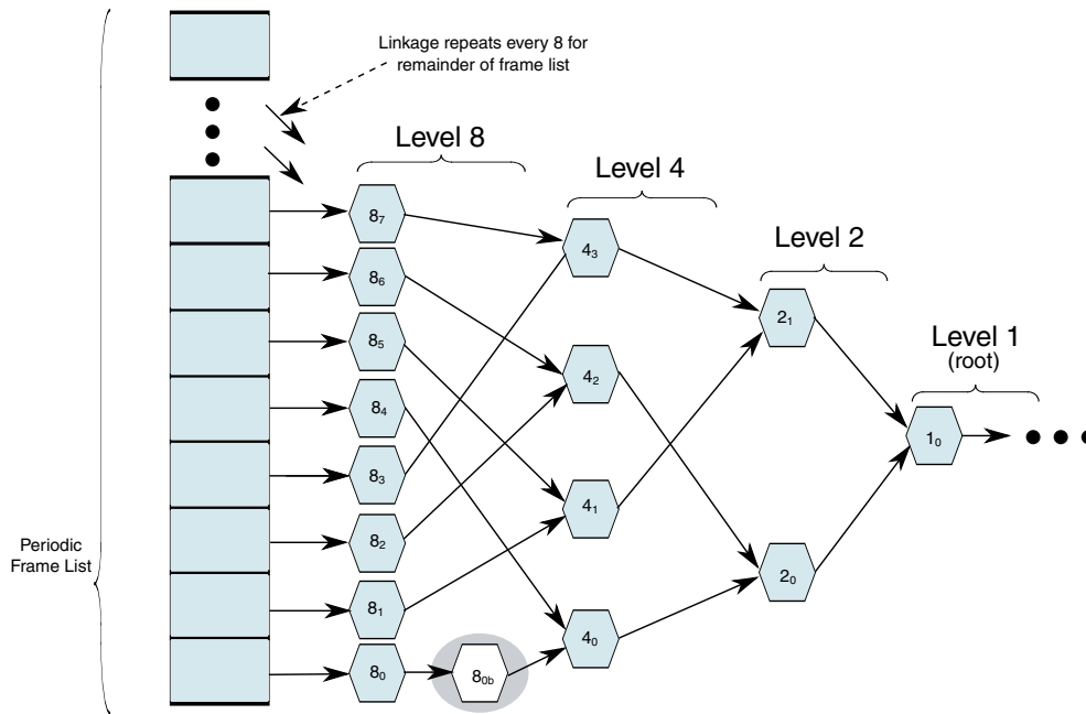
Figure 43-159. General Structure of EHCI Periodic Schedule Utilizing Interrupt Spreading
