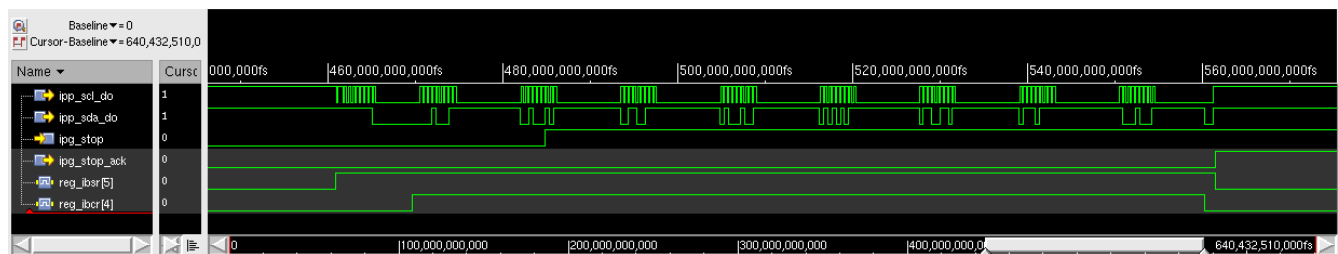
Figure 48-43. I 2 C stop mode behavior when master is receiving and slave is transmitting
