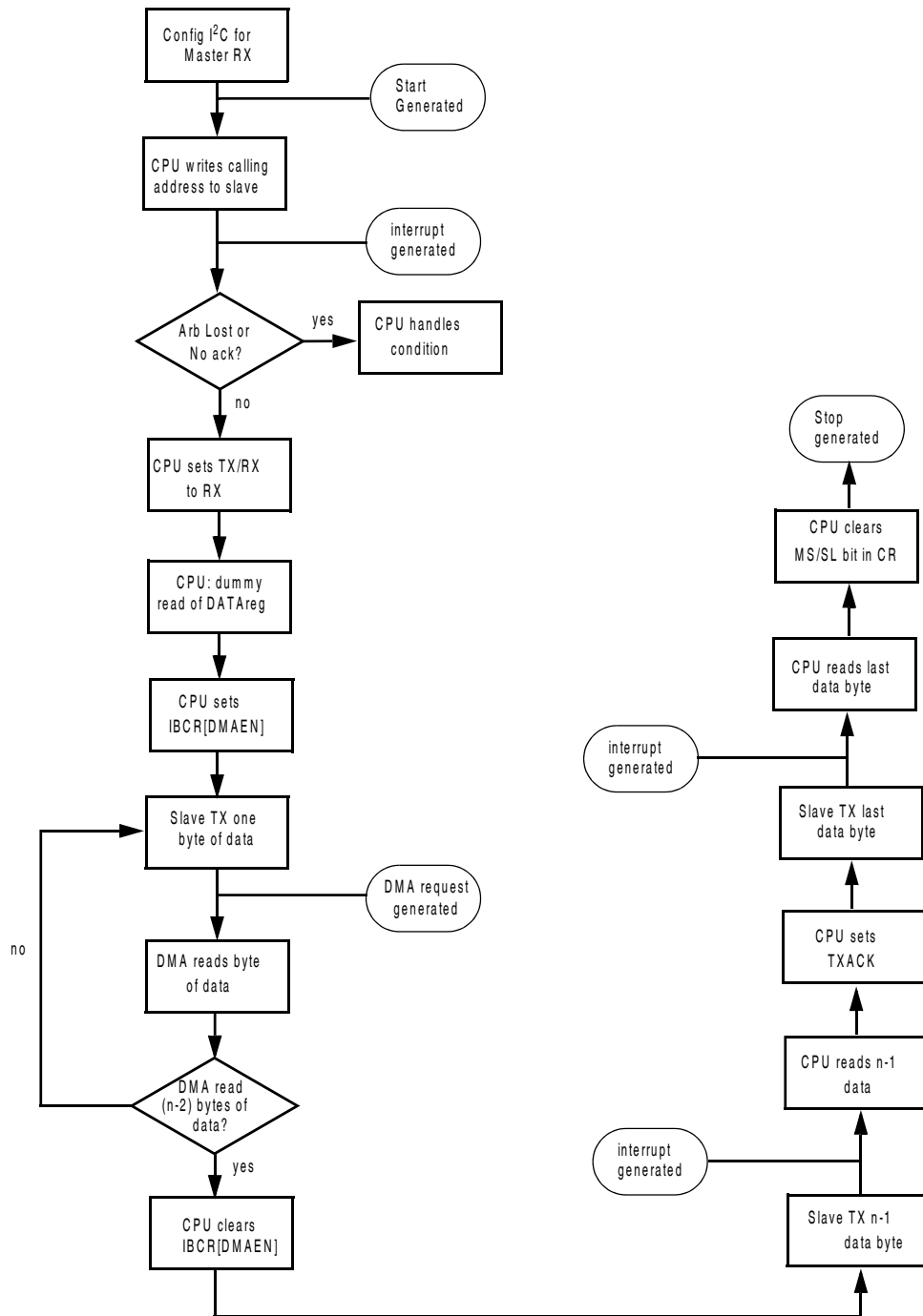
Figure 48-50. Flow-Chart of DMA mode master receive
