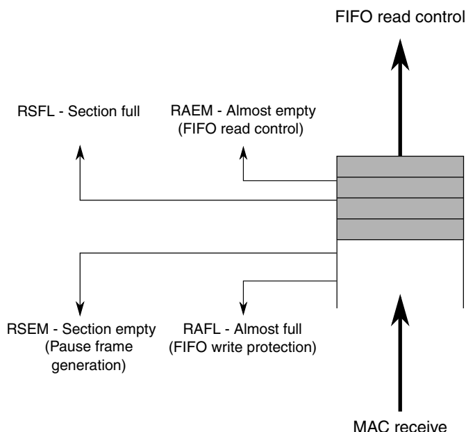
Figure 42-311. Receive FIFO overview
