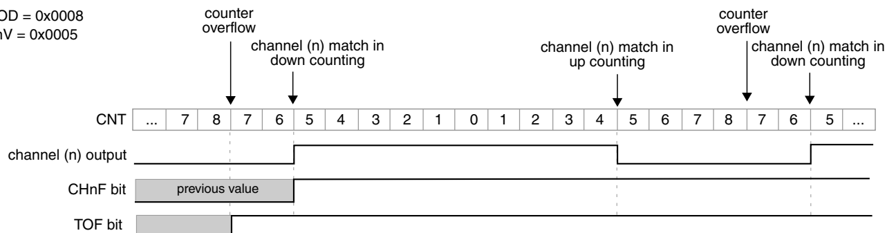
Figure 39-226. CPWM signal with ELSnB:ELSnA = 1:0
