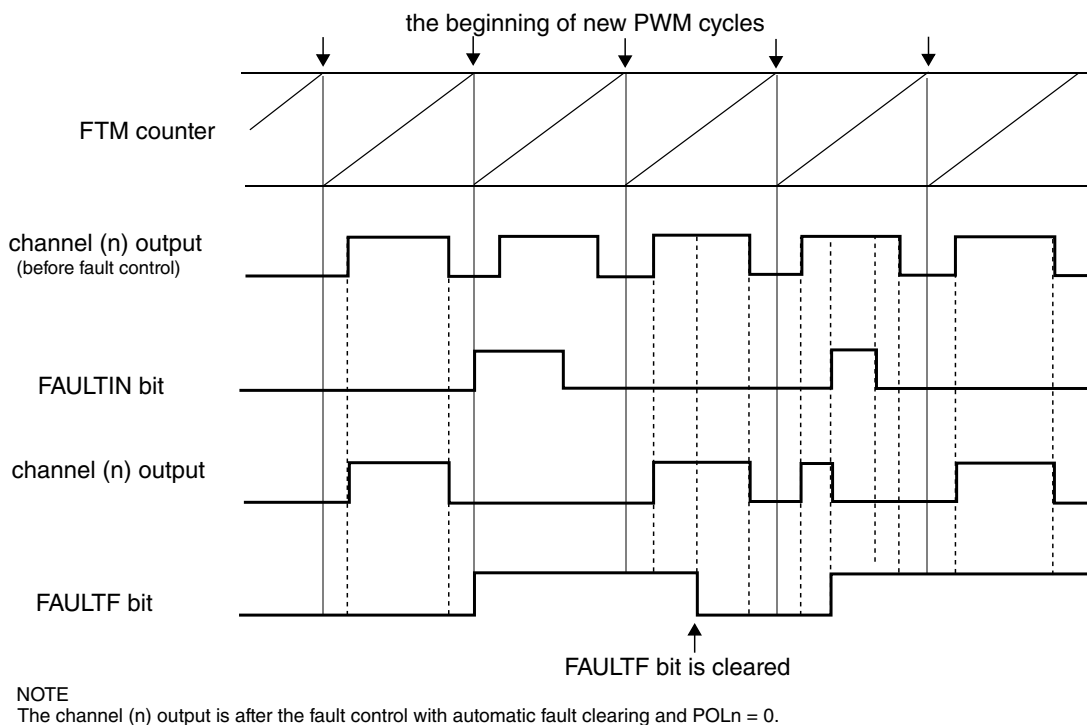
Figure 39-276. Fault control with automatic fault clearing
