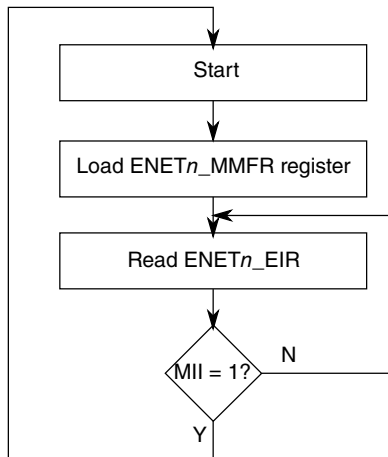
Figure 42-318. MDIO access overview
