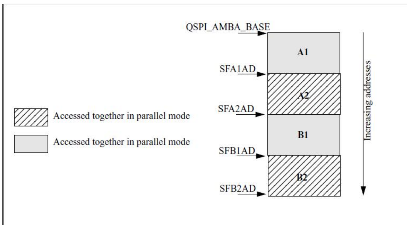
Figure 30-417. Flash addressing
