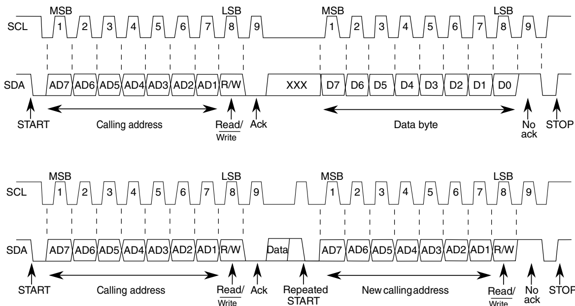
Figure 48-39. I 2 C transaction protocol
