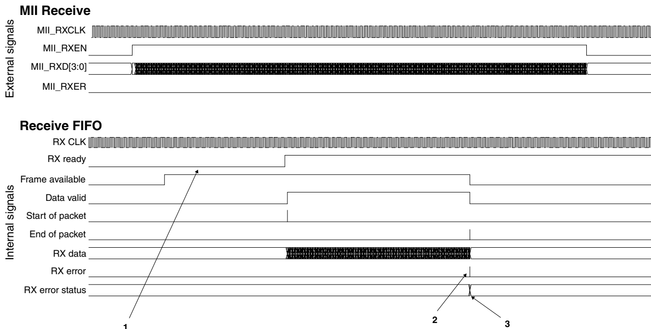
Figure 42-317. Receive FIFO overflow protection
