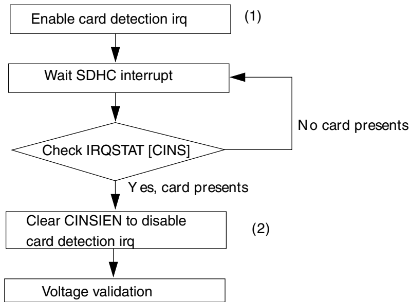
Figure 50-87. Flow diagram for card detection
