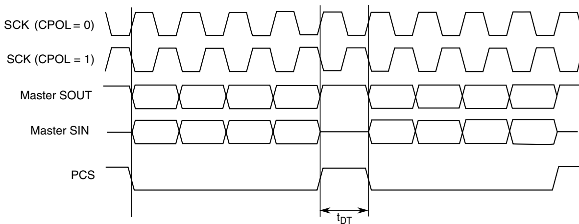
Figure 47-131. Continuous SCK Timing Diagram (CONT=0)
