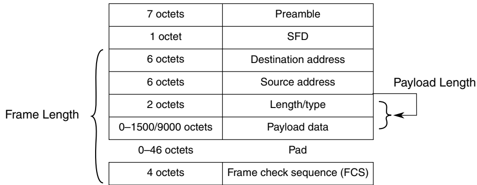
Figure 42-302. MAC frame format overview
