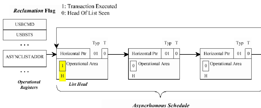
Figure 43-152. Asynchronous Schedule List w/Annotation to Mark Head of List
