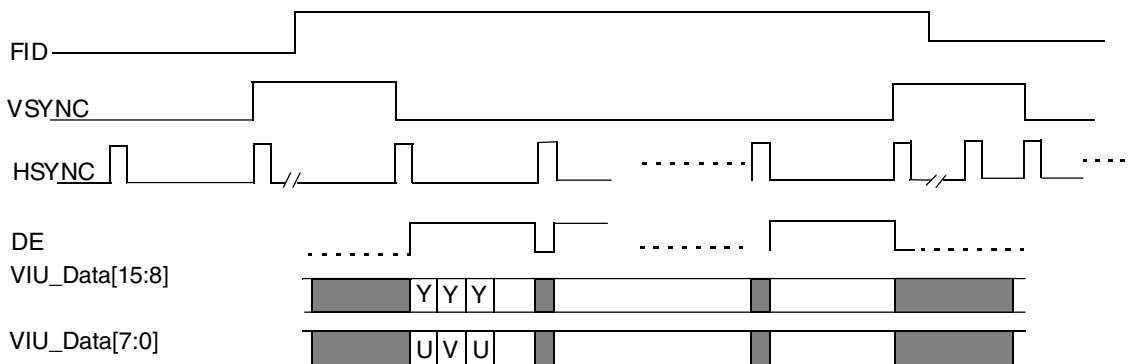
Figure 57-23. Parallel YC Timing
