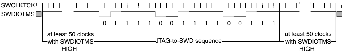
Figure 20-3. JTAG-to-SWD switching sequence
