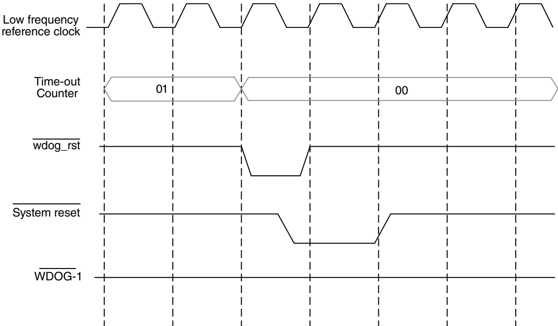
Figure 26-3. WDOG timeout condition/WDT bit is not set
