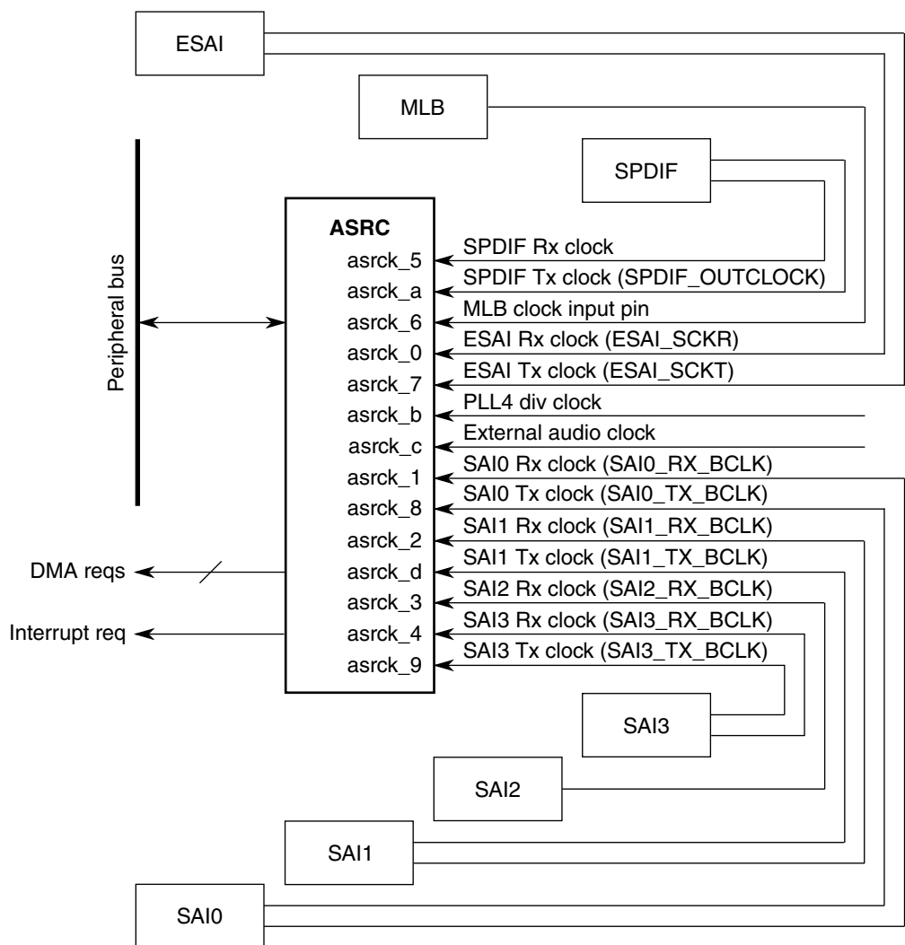
Figure 53-1. System Overview
