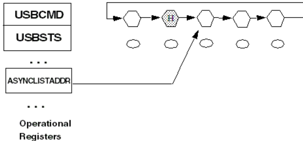
Figure 43-145. General Format of Asynchronous Schedule List
