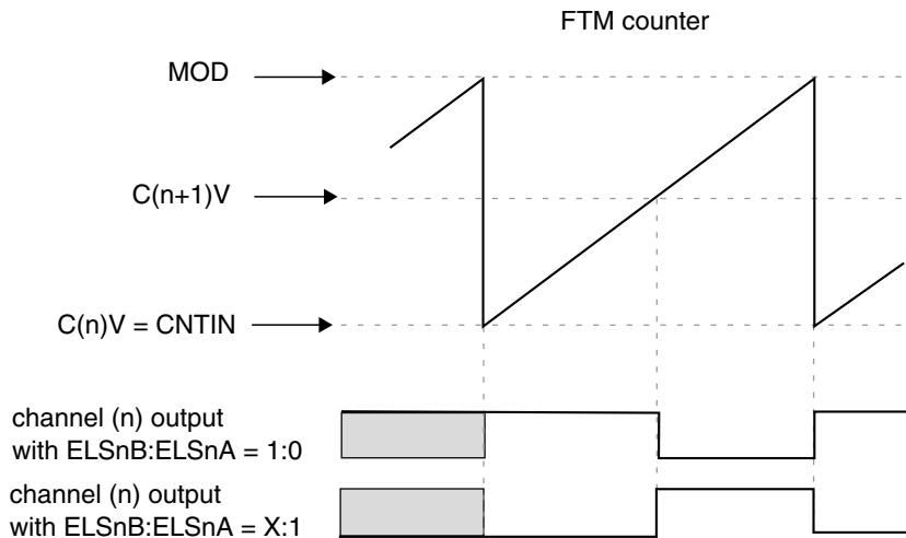
Figure 39-231. Channel (n) output if (C(n)V = CNTIN) and (CNTIN < C(n+1)V < MOD)
