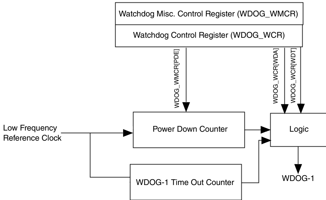
Figure 26-2. WDOG_B generation
