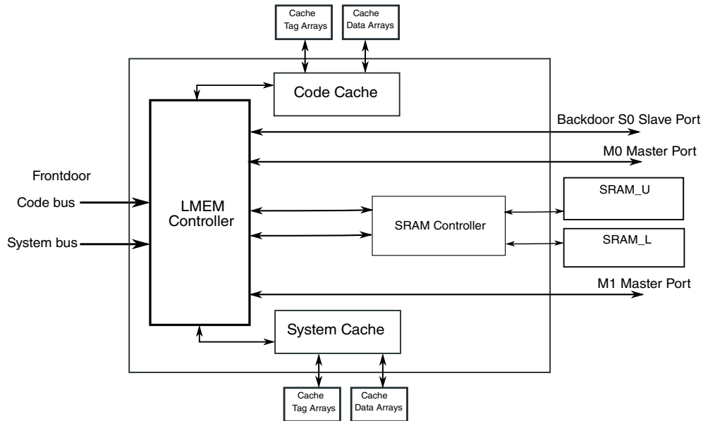
Figure 29-10. SRAM Configuration
