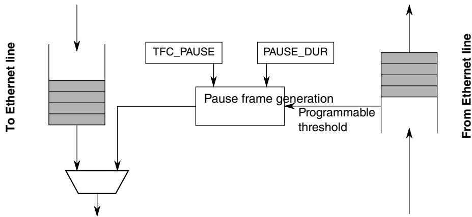
Figure 42-308. Pause frame generation overview
