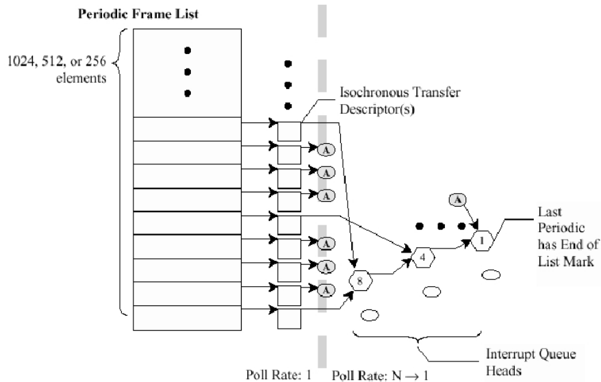
Figure 43-149. Example Periodic Schedule
