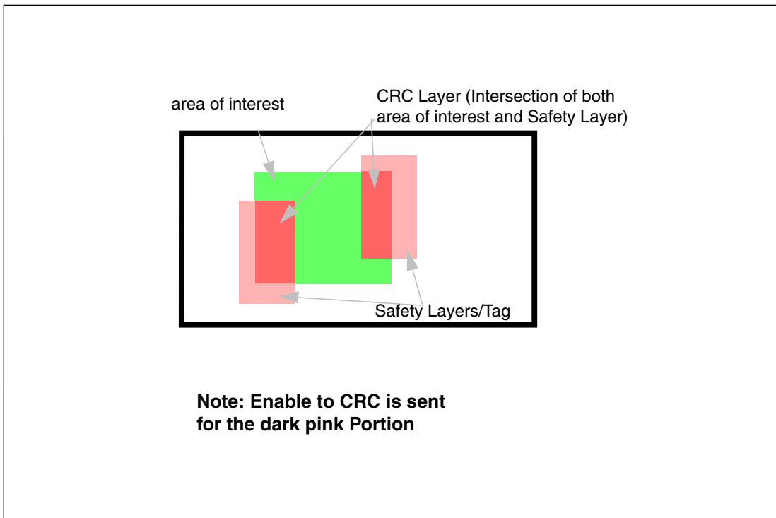
Figure 55-1947. Safety Mode with tag bit high
