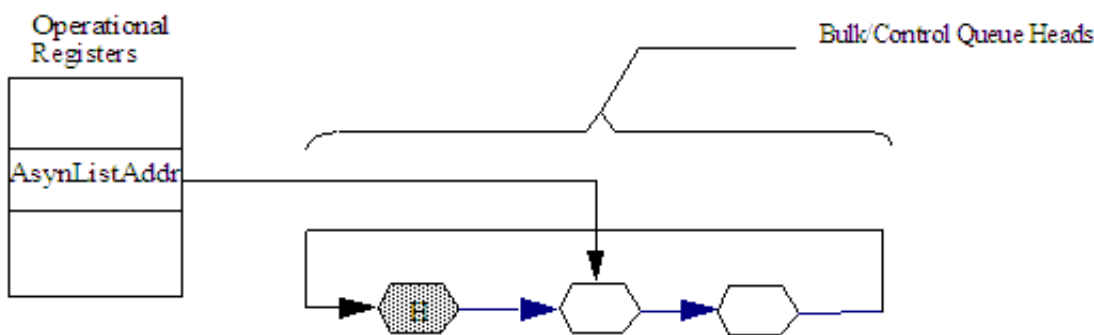
Figure 43-141. Asynchronous schedule organization
