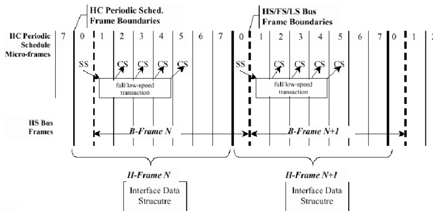
Figure 43-148. Relationship of Periodic Schedule Frame Boundaries to Bus Frame Boundaries
