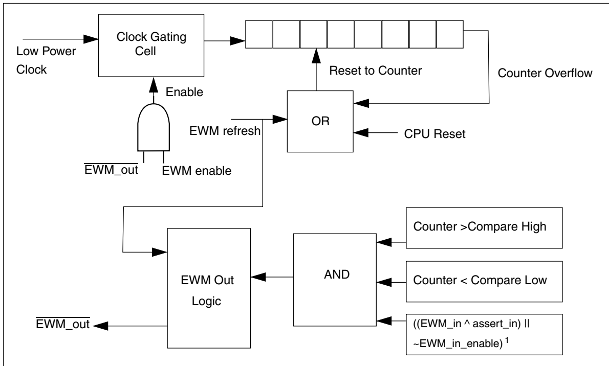
Figure 25-1. EWM Block Diagram
