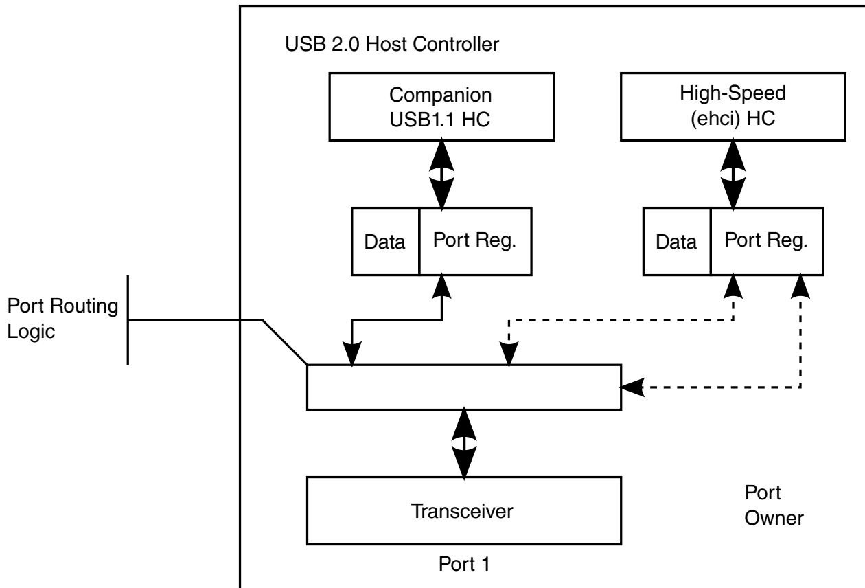
Figure 43-142. Example USB 2.0 Host Controller Port Routing Block Diagram
