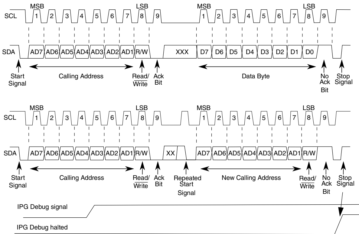
Figure 48-47. IPG debug mode with repeated start
