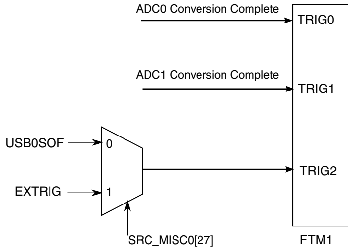
Figure 3-7. FTM1 Triggers
