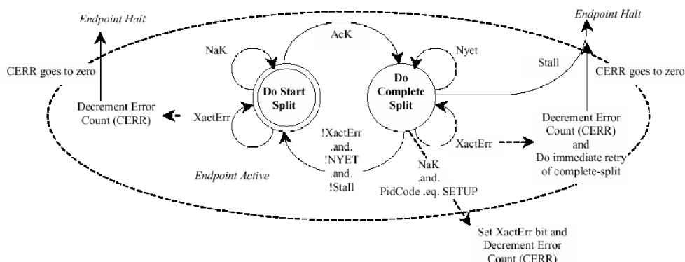
Figure 43-157. Host Controller Asynchronous Schedule Split-Transaction State Machine
