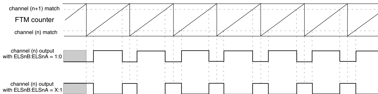
Figure 39-228. Combine mode
