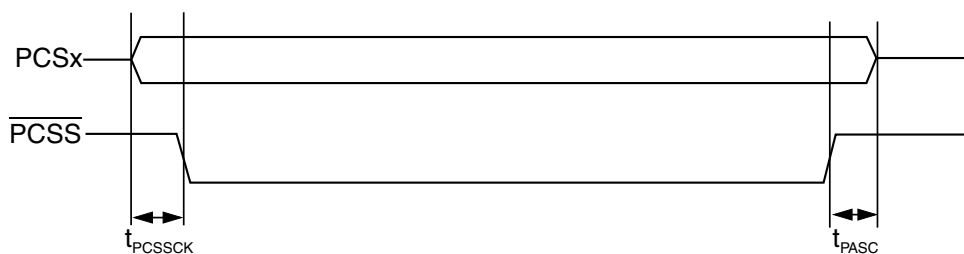
Figure 47-125. Peripheral Chip Select Strobe timing
