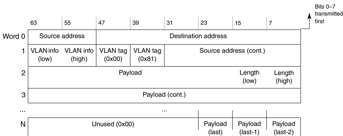
Figure 42-315. VLAN-tagged frame 64-bit mapping example
