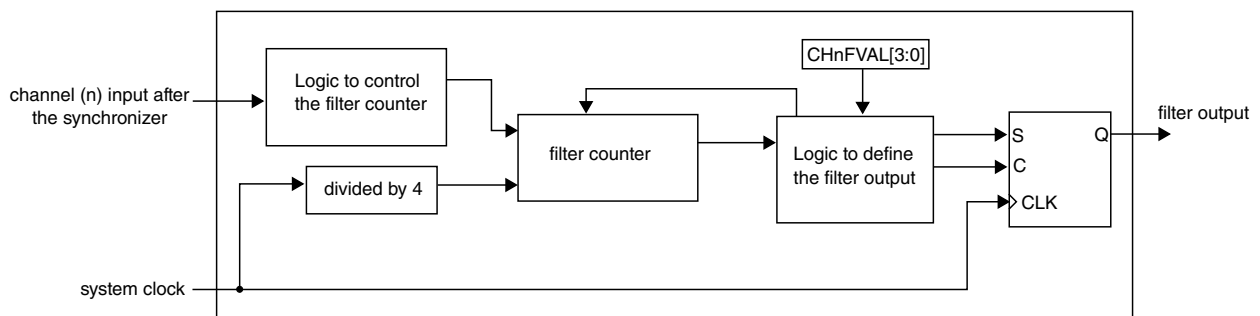
Figure 39-217. Channel input filter
