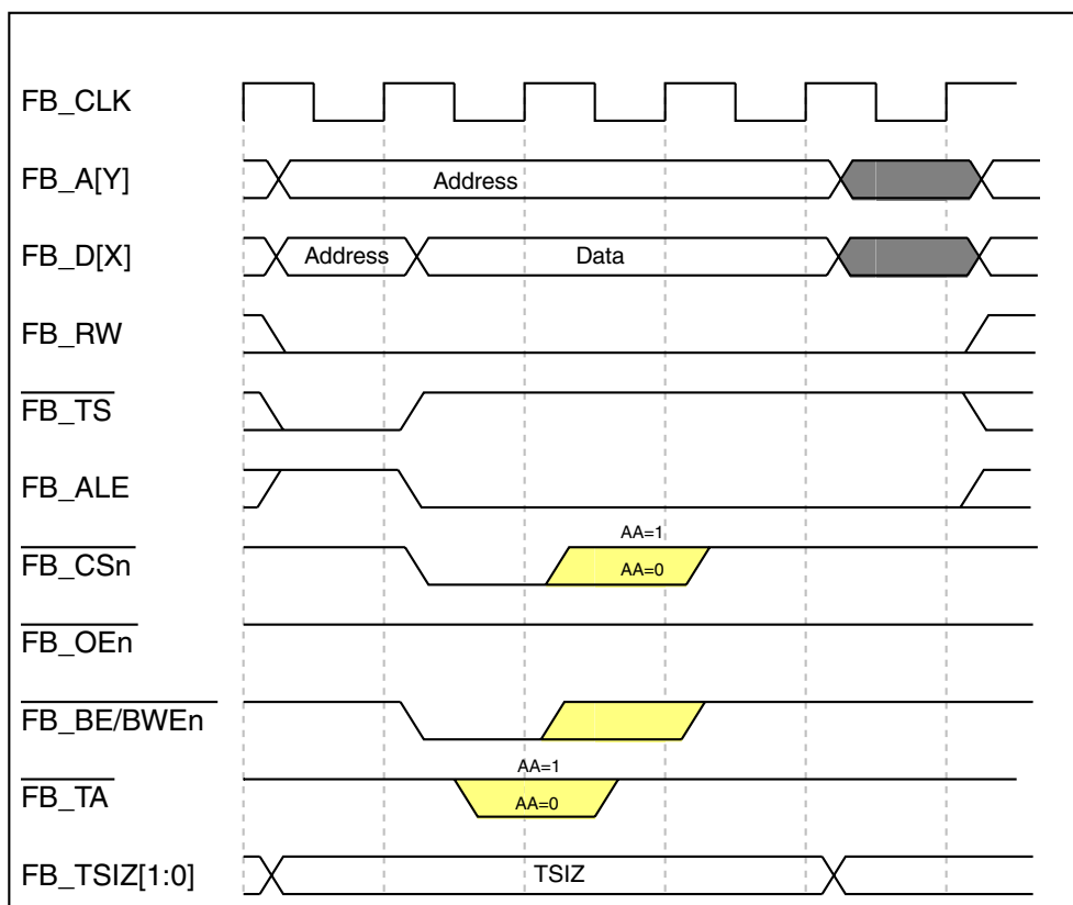
Figure 32-39. Write Cycle with Two-Clock Address Hold (No Wait States)
