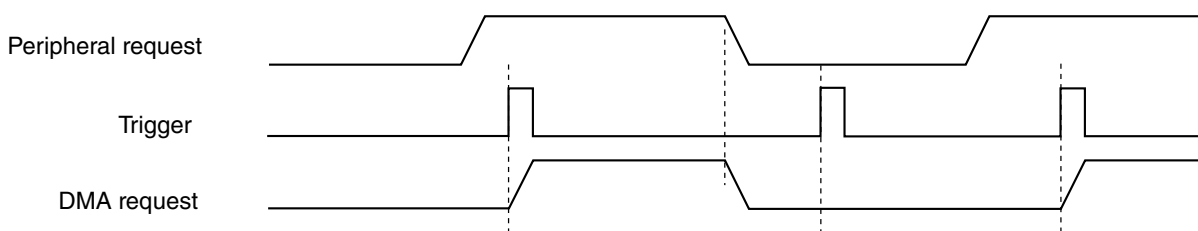
Figure 22-89. DMAMUX channel triggering: ignored trigger
