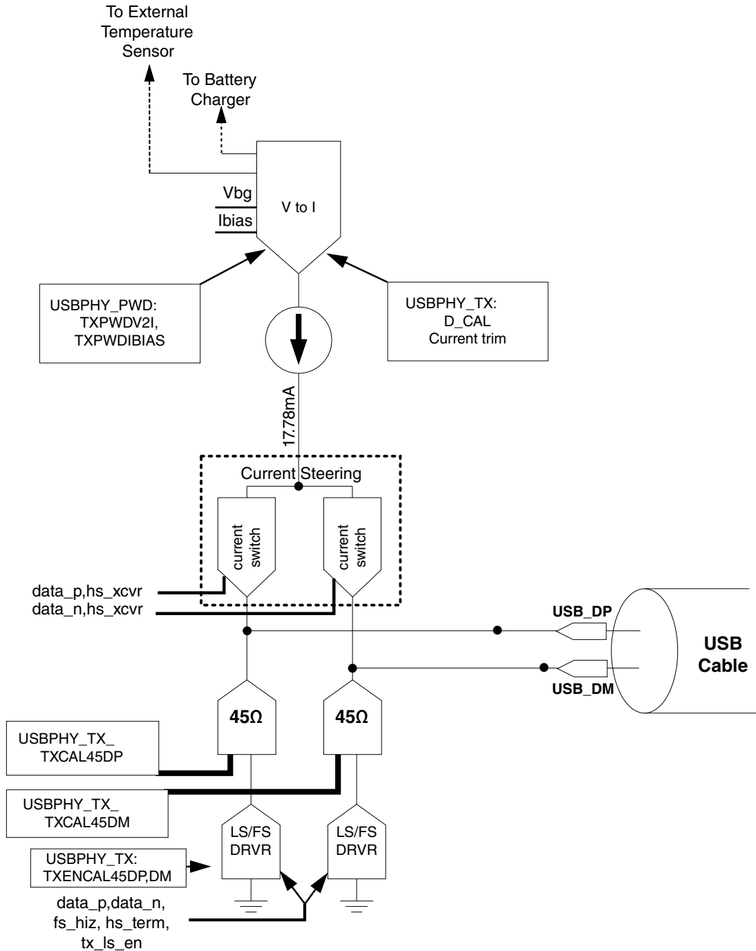
Figure 44-117. USB 2.0 PHY Transmitter Block Diagram
