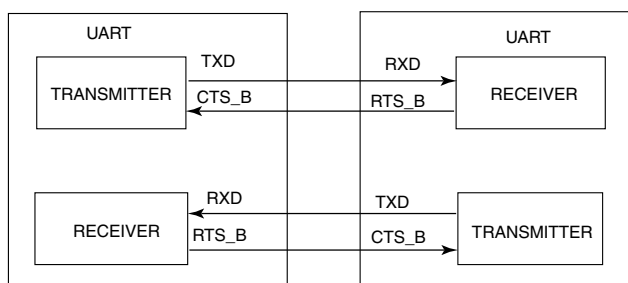
Figure 49-245. Ready-to-receive
