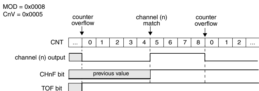
Figure 39-224. EPWM signal with ELSnB:ELSnA = X:1
