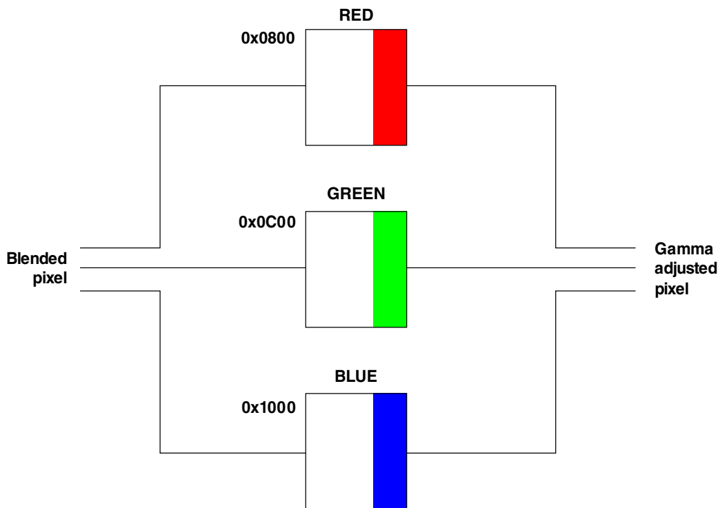
Figure 55-1942. Gamma Correction Table Organization
