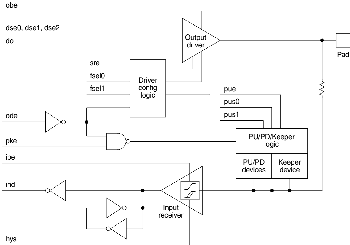
Figure 6-235. GPIO PAD
