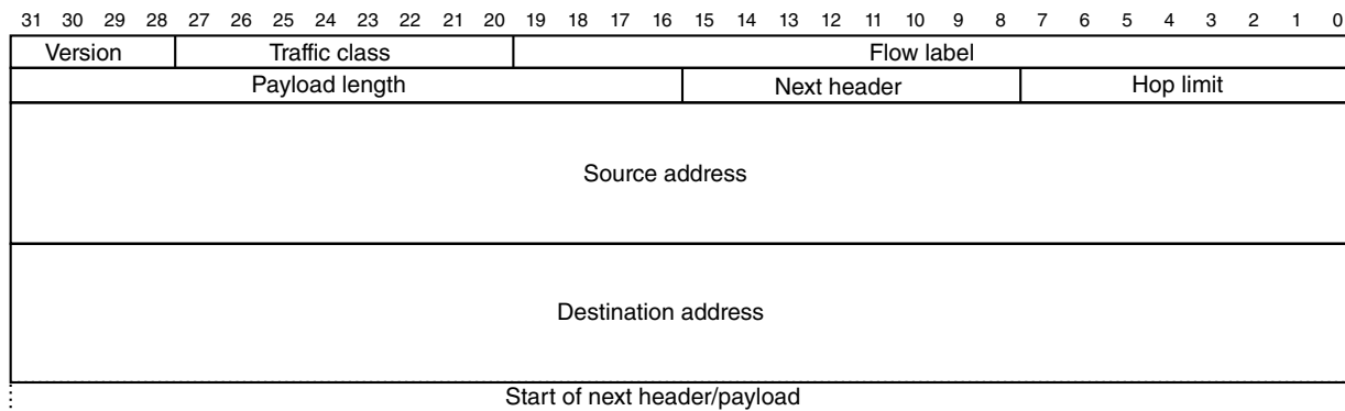
Figure 42-304. IPv6 header format
