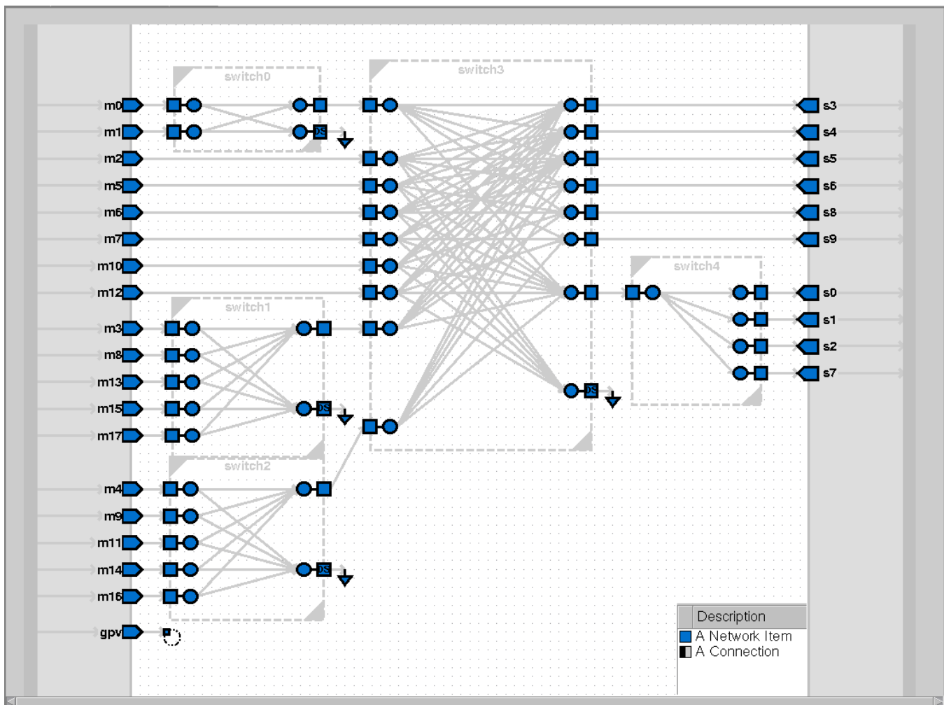
Figure 63-2. NIC301 Physical Block Diagram
