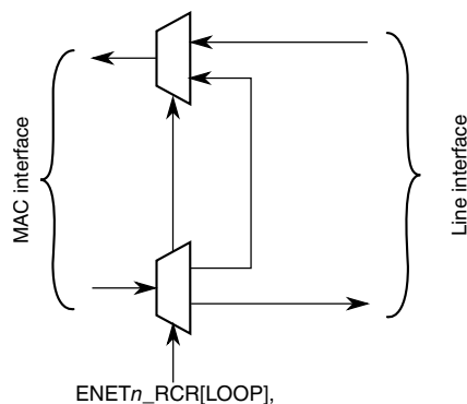
Figure 42-313. Loopback options
