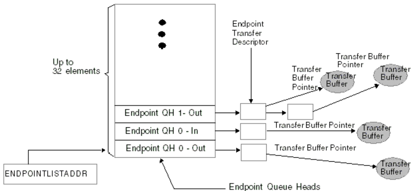
Figure 43-165. End Point Queue Head Organization
