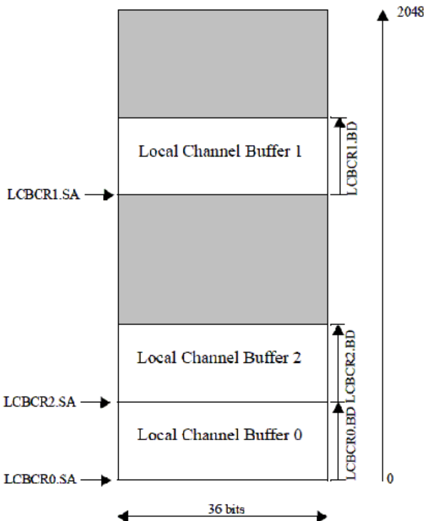
Figure 45-97. Programming Example for LCBCRn
