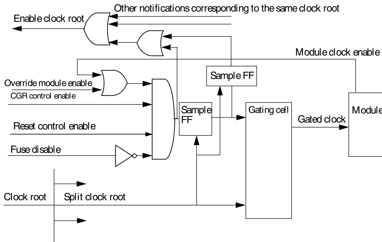
Figure 10-45. Implementation for each gating cell
