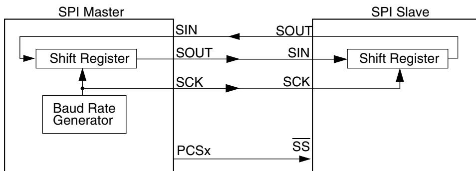
Figure 47-123. Serial protocol overview
