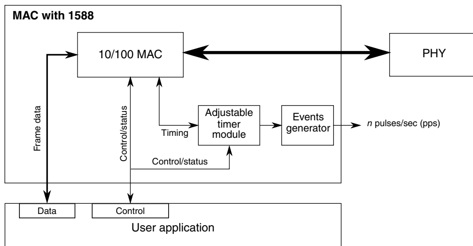
Figure 42-309. IEEE 1588 functions overview
