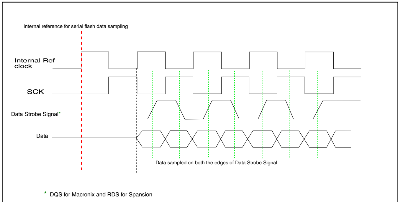
Figure 30-423. Data strobe signal functionality
