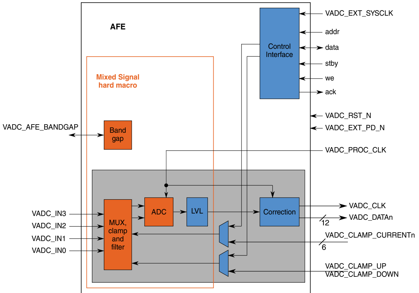
Figure 61-2. Analog front end block diagram
