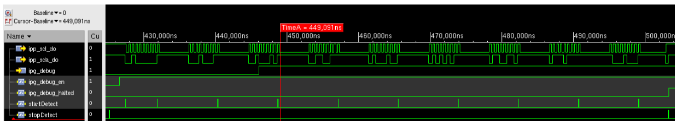
Figure 48-44. Simulation result of IPG Debug Halted in case of frame transmission
