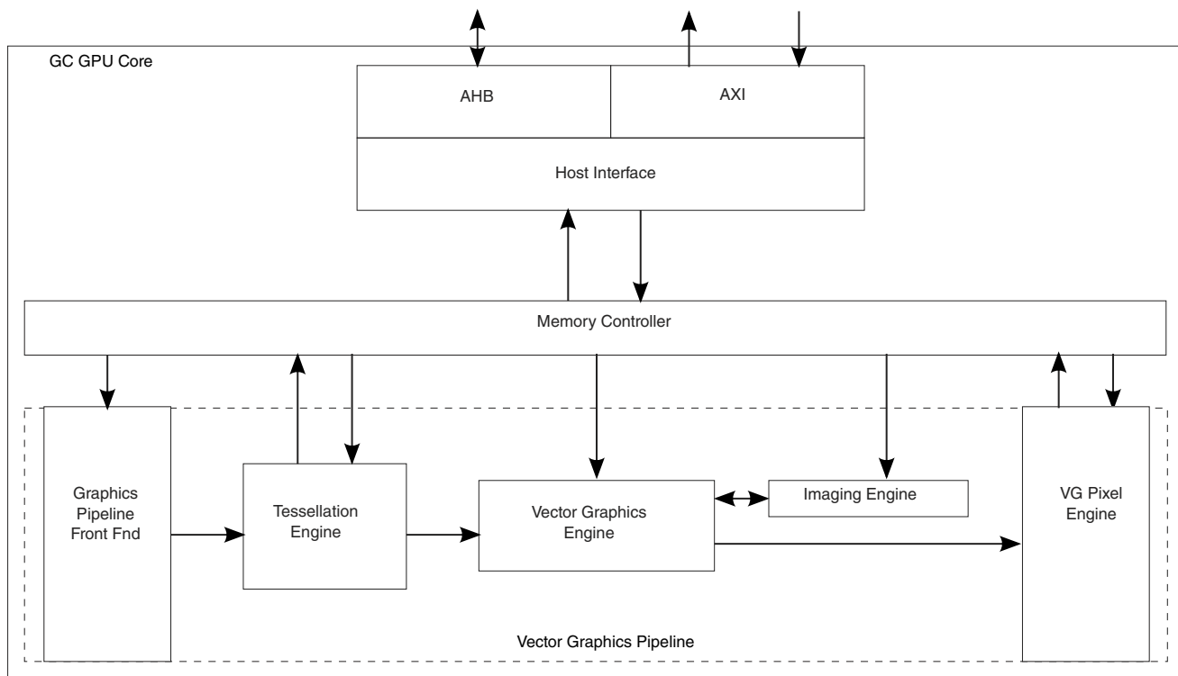
Figure 60-1. Module Block Diagram
