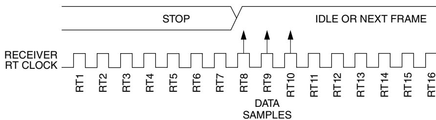
Figure 49-230. Fast data
