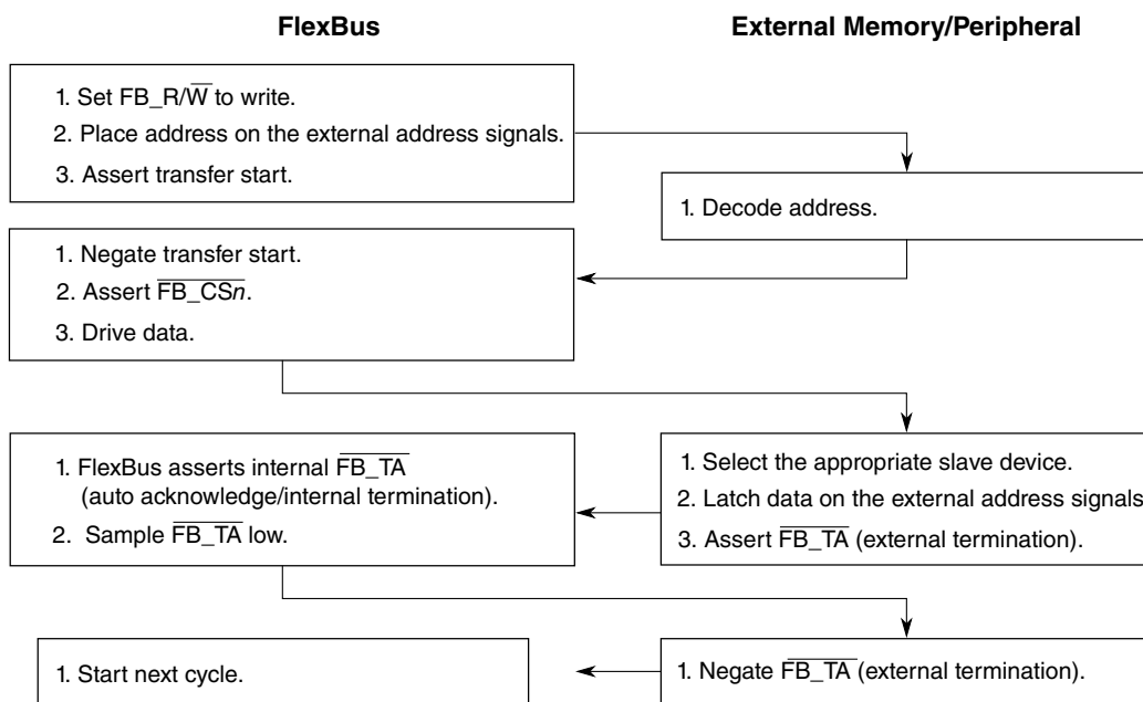
Figure 32-24. Write-Cycle Flowchart
