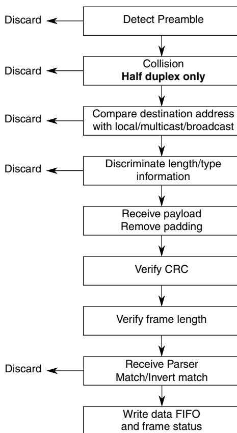
Figure 42-305. MAC receive flow
