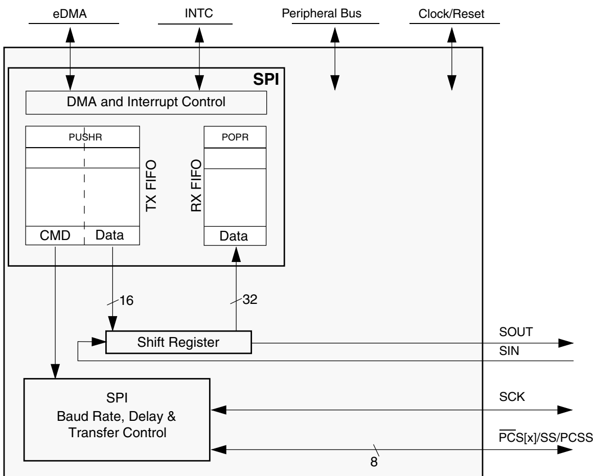
Figure 47-1. SPI Block Diagram
