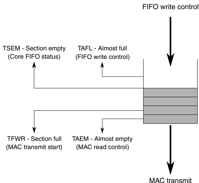
Figure 42-312. Transmit FIFO overview
