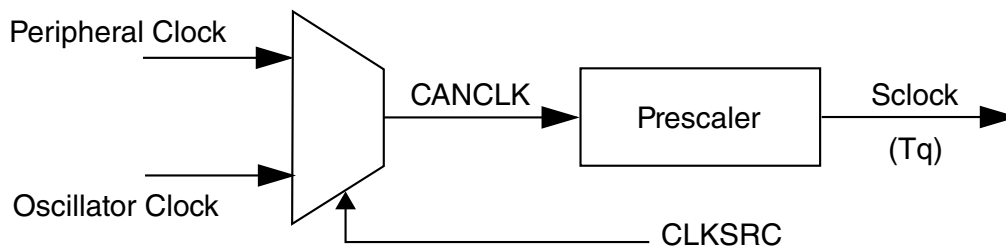
Figure 46-272. CAN engine clocking scheme
