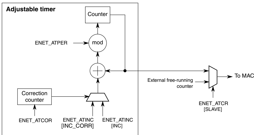
Figure 42-310. Adjustable timer implementation detail
