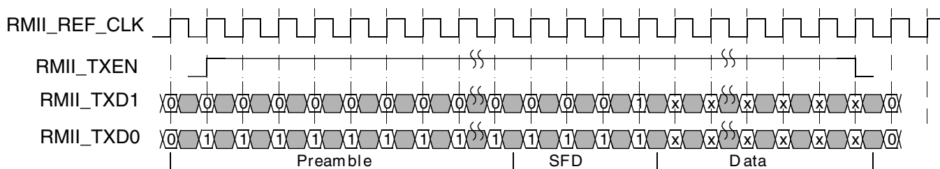
Figure 42-321. RMIi transmit operation
