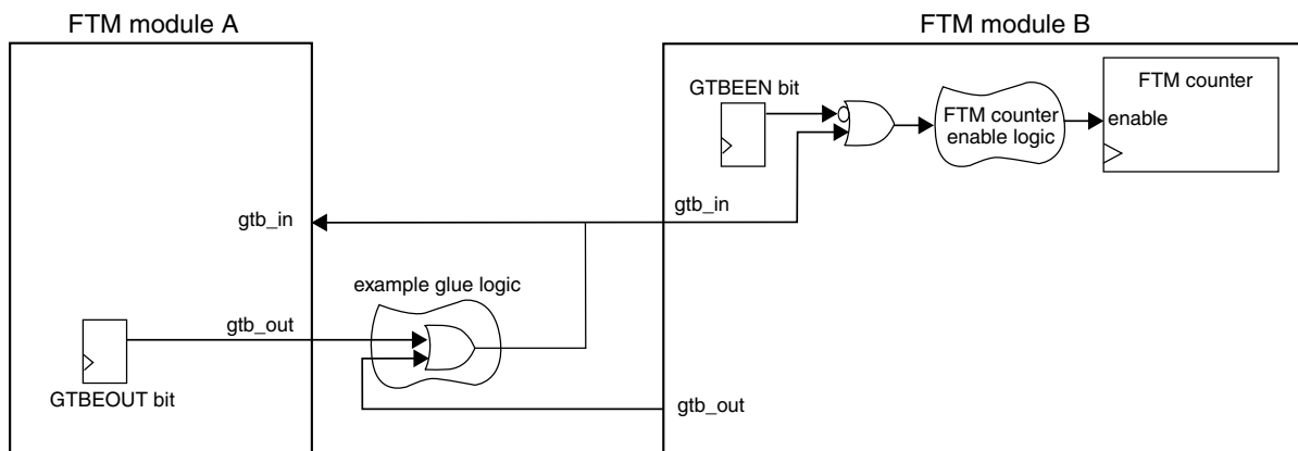
Figure 39-299. Global time base (GTB) block diagram
