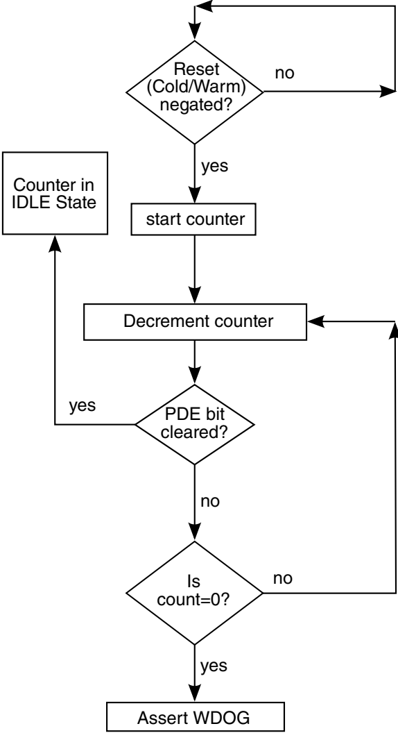
Figure 26-5. Power-Down Counter Flow Diagram
