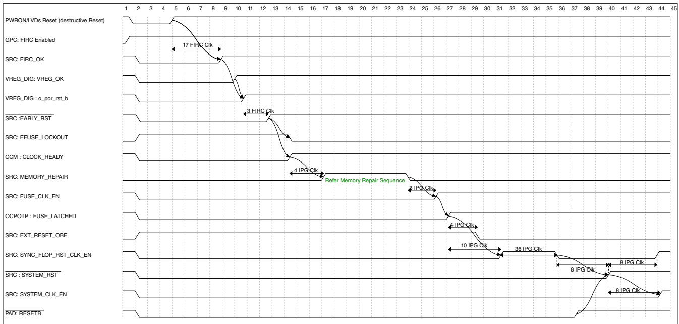
Figure 18-20. Destructive reset sequence
