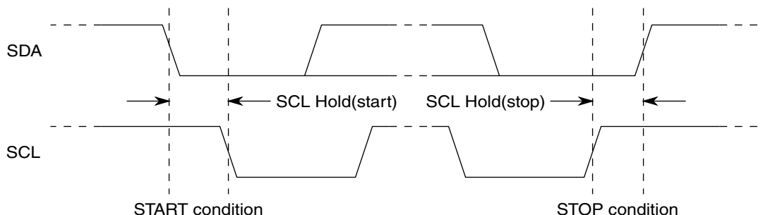
Figure 48-42. SCL Divider and SDA Hold
