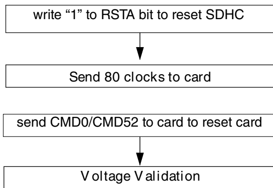
Figure 50-88. Flow chart for reset of the SDHC and SD I/O card
