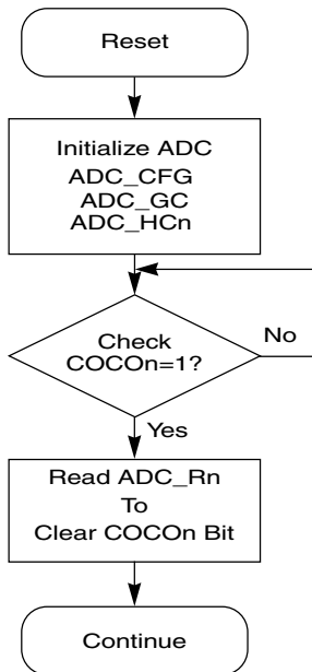
Figure 37-40. Initialization Flowchart for Example
