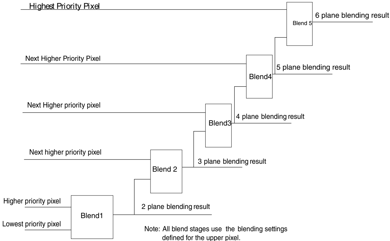
Figure 55-1923. Pixel blending stack
