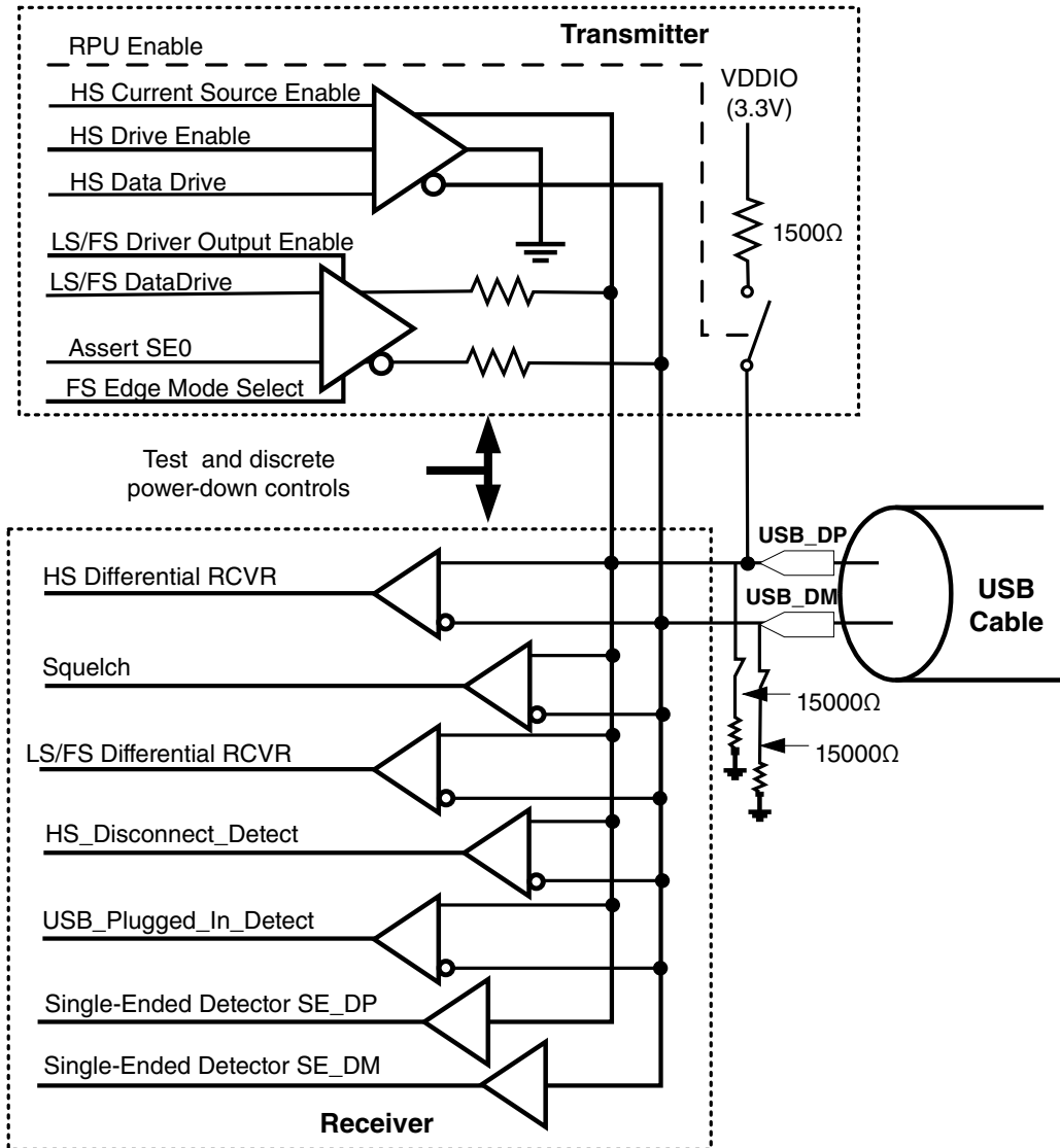
Figure 44-116. USB 2.0 PHY Analog Transceiver Block Diagram
