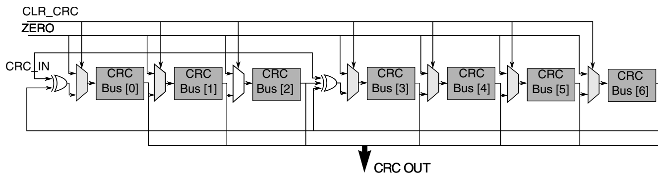
Figure 50-82. Command CRC Shift Register
