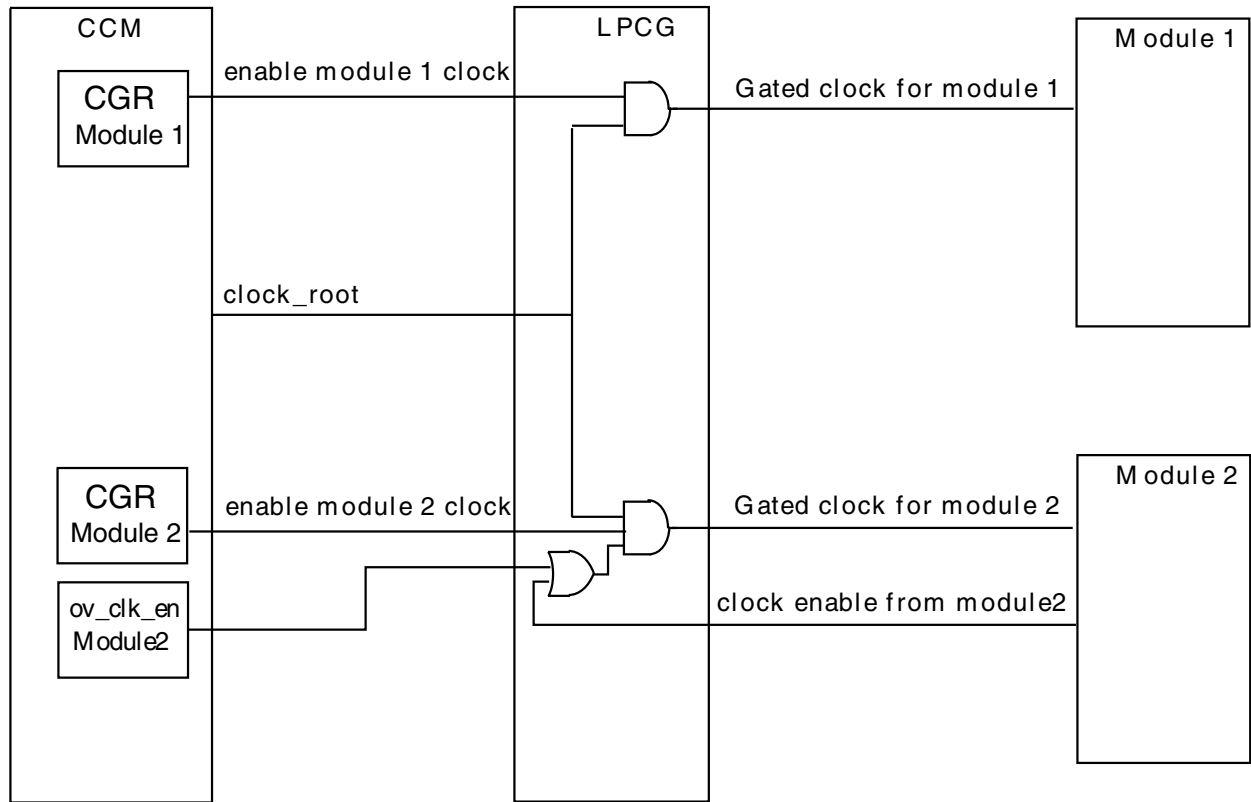
Figure 10-46. Power Modes
