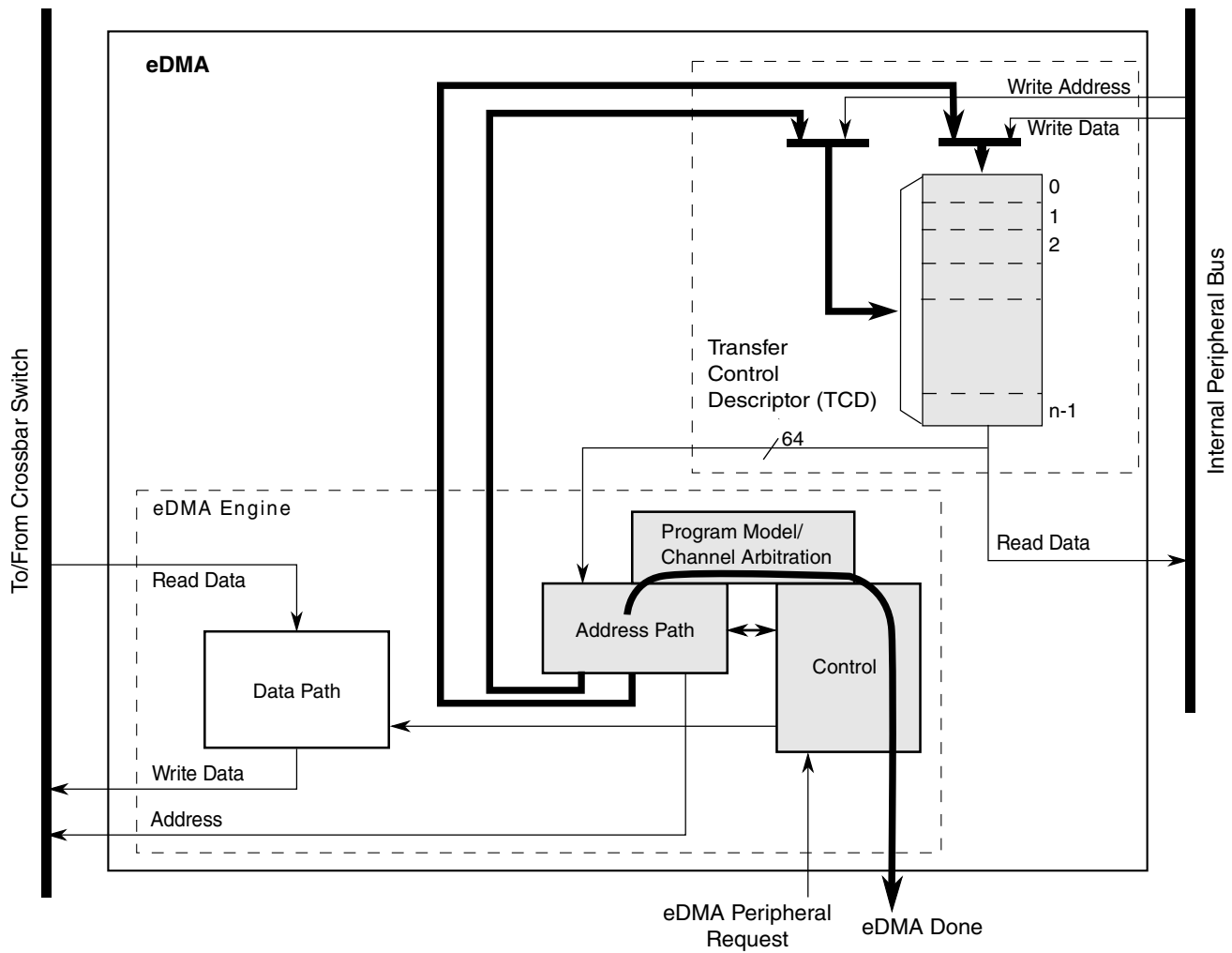
Figure 21-1636. eDMA operation, part 3
