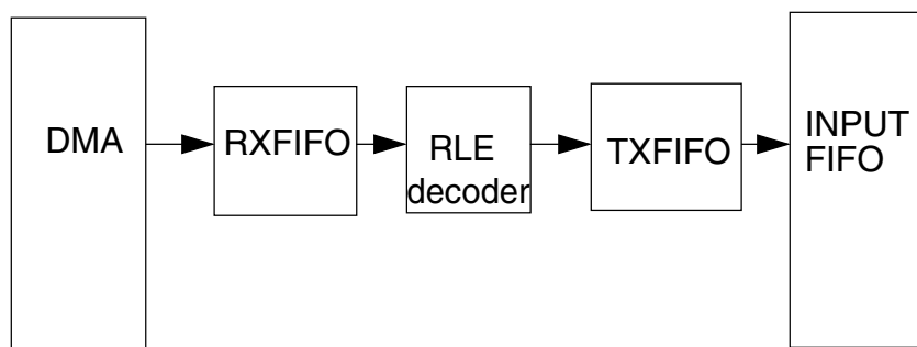
Figure 55-1944. RLE Decoding in DCU5
