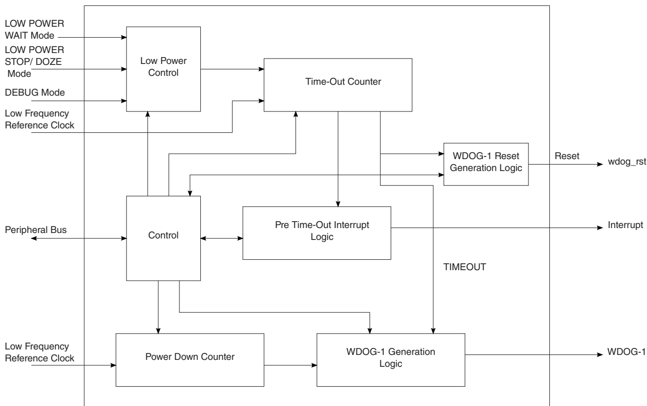
Figure 26-1. WDOG Diagram
