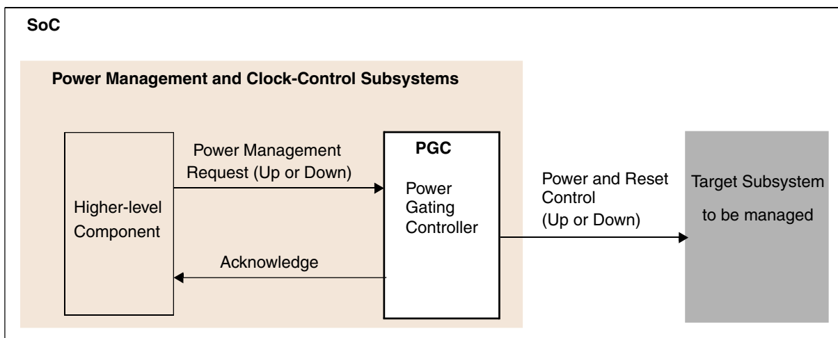
Figure 15-6. PGC Top-Level Block Diagram
