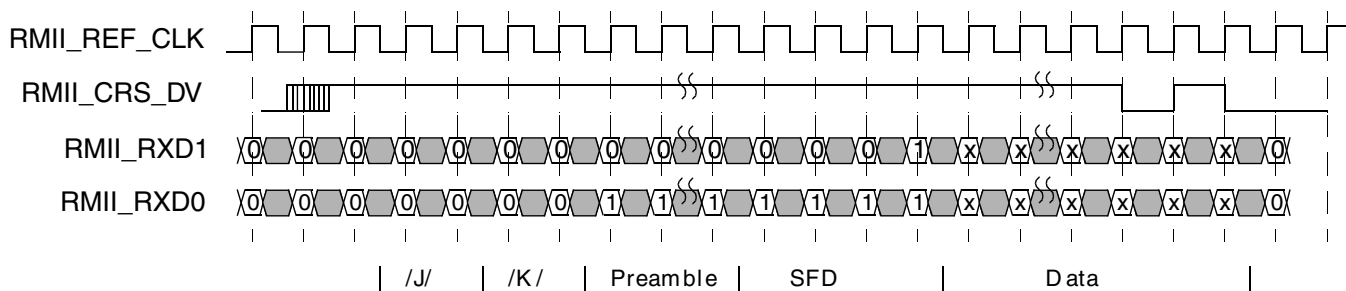
Figure 42-319. RMIi receive operation
