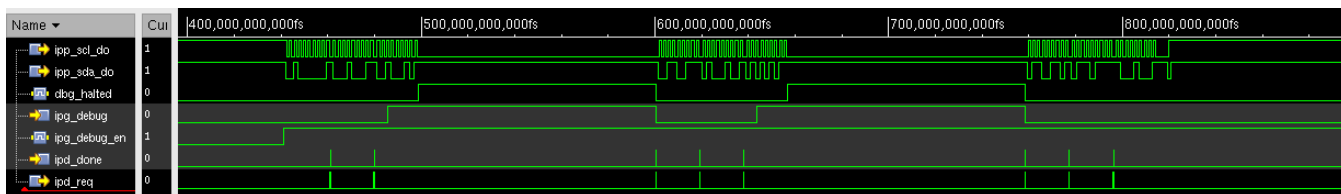
Figure 48-45. Simulation result of IPG Debug Halted in case of frame transmission using DMA
