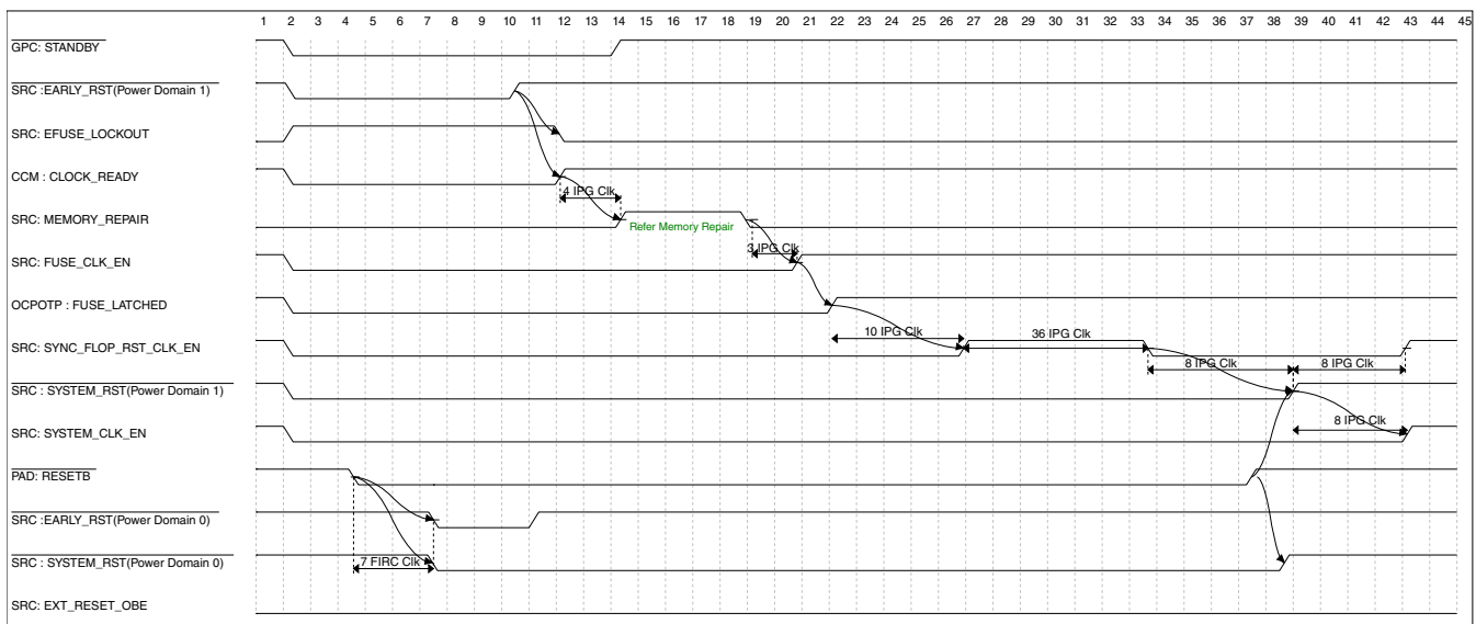
Figure 18-24. Standby reset sequence (Abort by External Reset)
