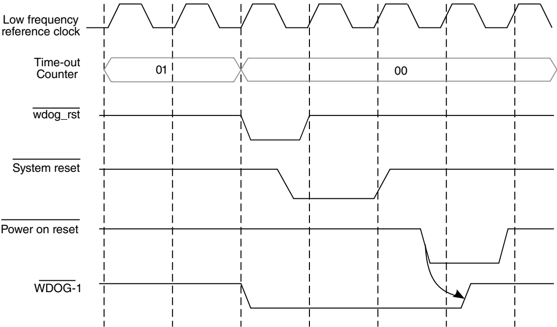
Figure 26-4. WDOG timeout condition/WDT bit is set
