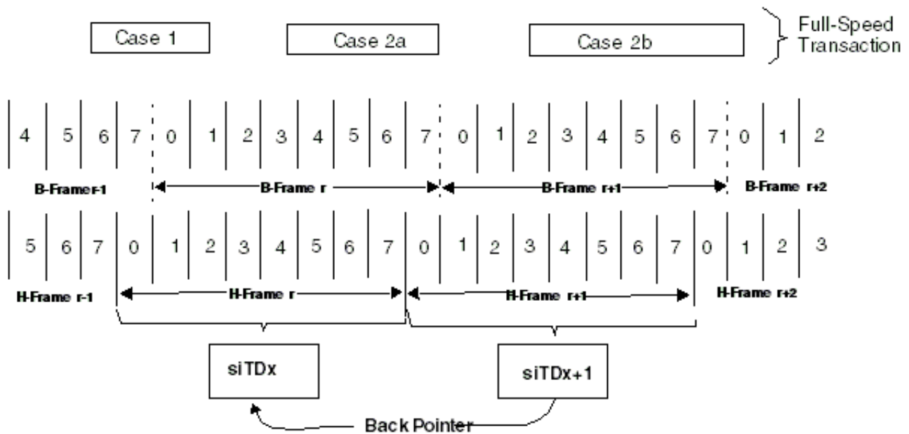
Figure 43-163. siTD Scheduling Boundary Examples
