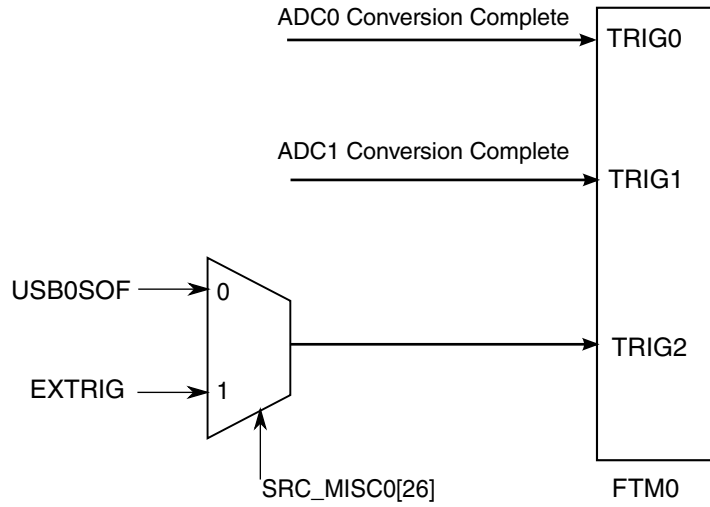
Figure 3-6. FTM0 Triggers
