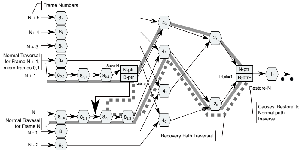
Figure 43-160. Example Host Controller Traversal of Recovery Path via FSTNs
