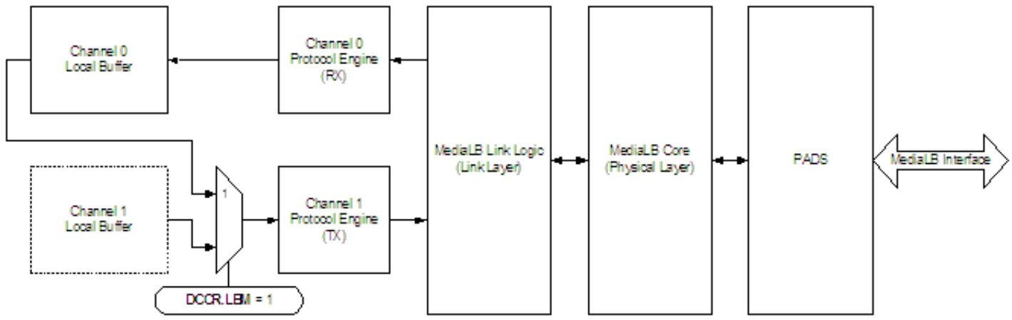
Figure 45-98. Loop-Back Test Mode Data Path
