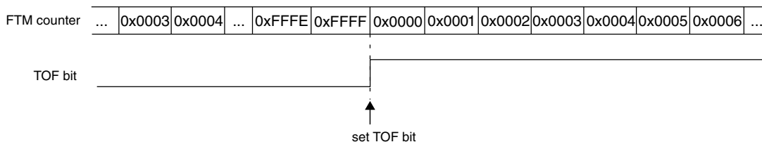
Figure 39-213. Example when the FTM counter is free running
