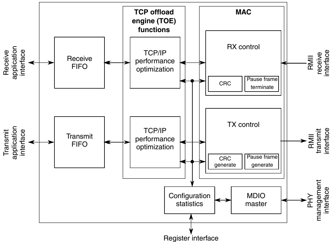
Figure 42-1. Ethernet MAC-NET core block diagram
