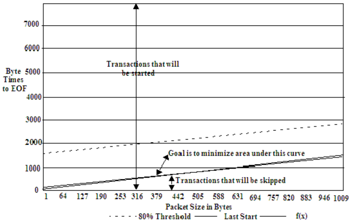
Figure 43-146. Best Fit Approximation
