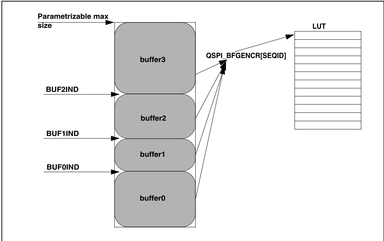
Figure 30-414. Flexible AHB Buffers
