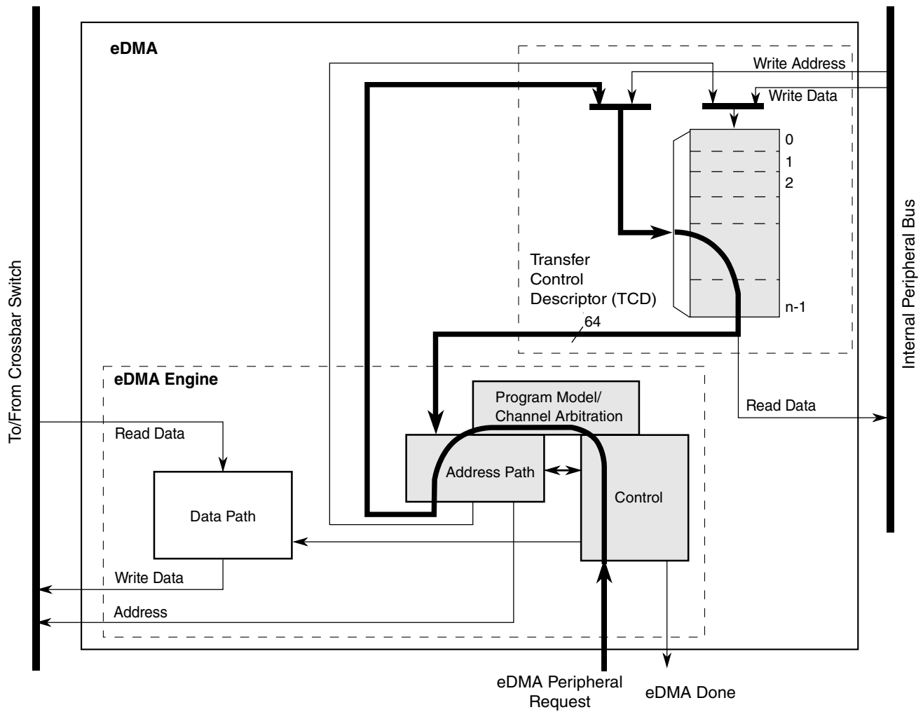
Figure 21-1634. eDMA operation, part 1
