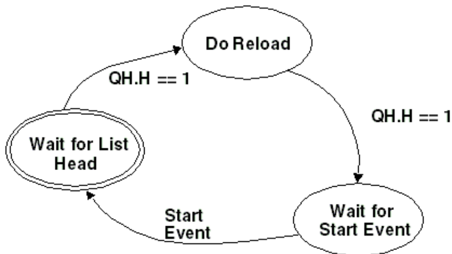
Figure 43-154. Example HC State Machine for Controlling Nak Counter Reloads
