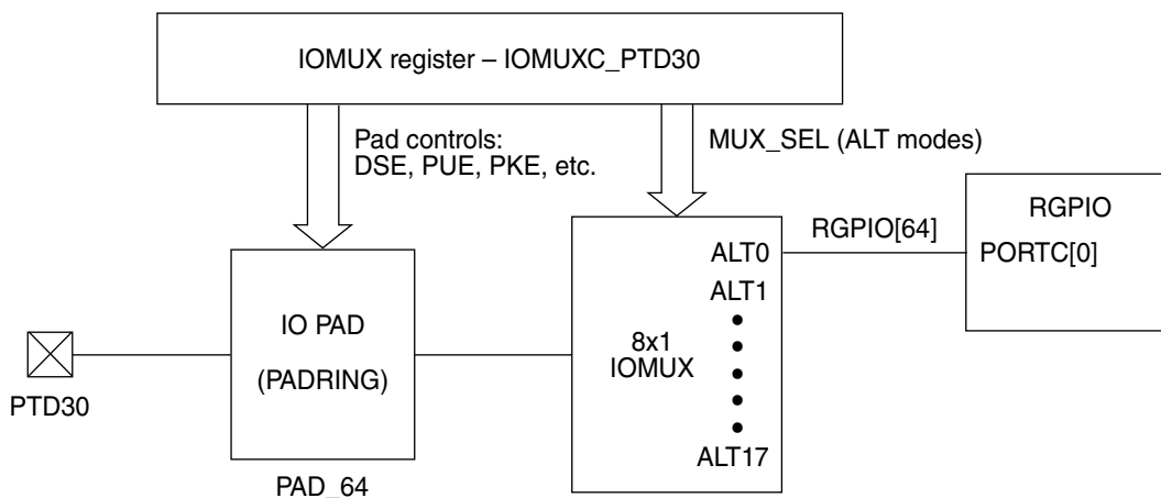
Figure 6-236. Path from the pint PTD30 to RGPIO
