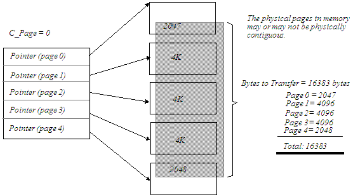
Figure 43-156. Example Mapping of qTD Buffer Pointers to Buffer Pages
