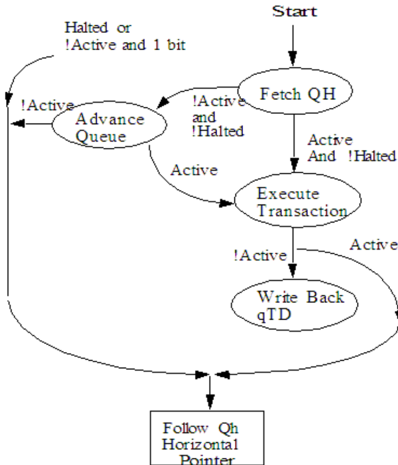
Figure 43-155. Host Controller Queue Head Traversal State Machine
