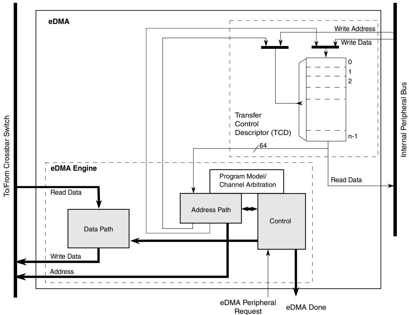
Figure 21-1635. eDMA operation, part 2
