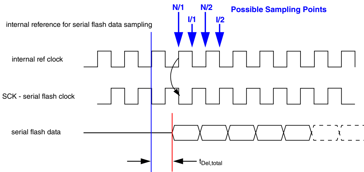
Figure 30-421. Serial Flash Sampling Clock Timing
