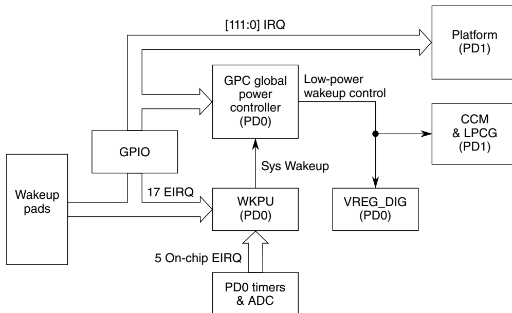
Figure 14-2. Interrupt connectivity
