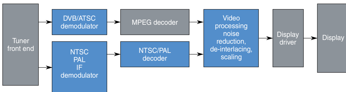
Figure 61-30. Video decoder block diagram
