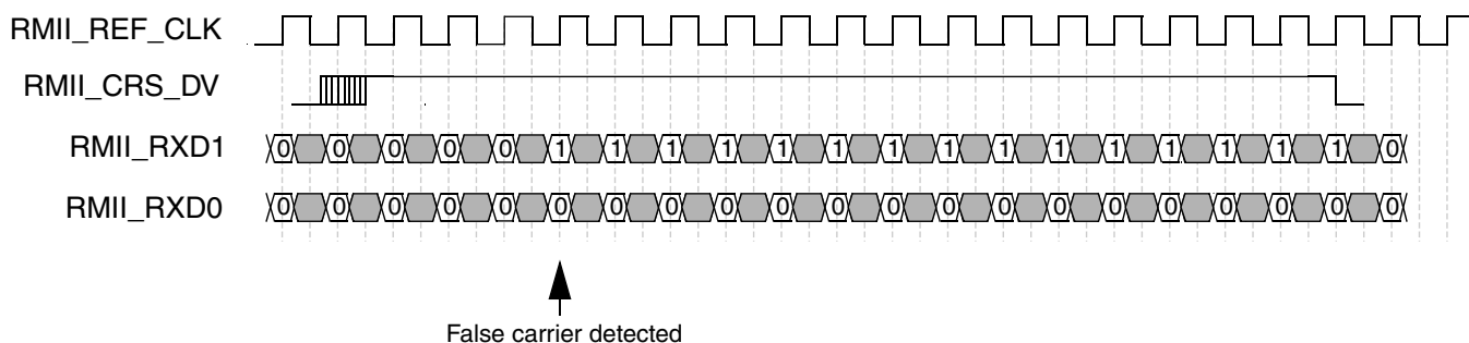
Figure 42-320. RMIi receive operation with false carrier
