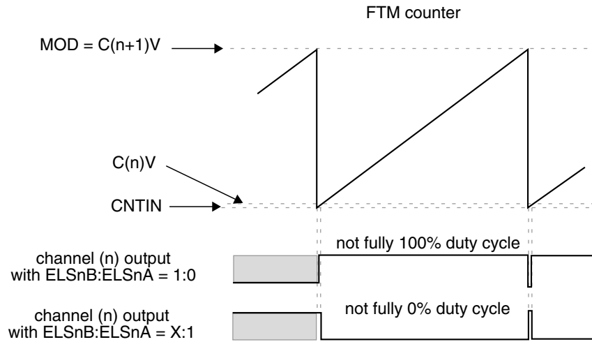
Figure 39-232. Channel (n) output if (CNTIN < C(n)V < MOD) and (C(n)V is Almost Equal to CNTIN ) and (C(n+1)V = MOD)
