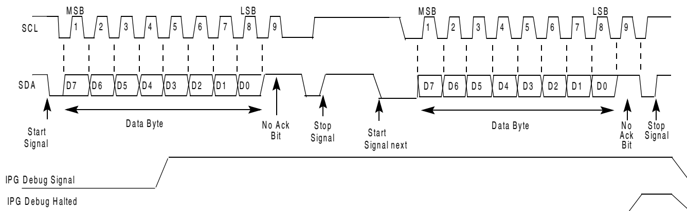
Figure 48-46. IPG DEBUG mode
