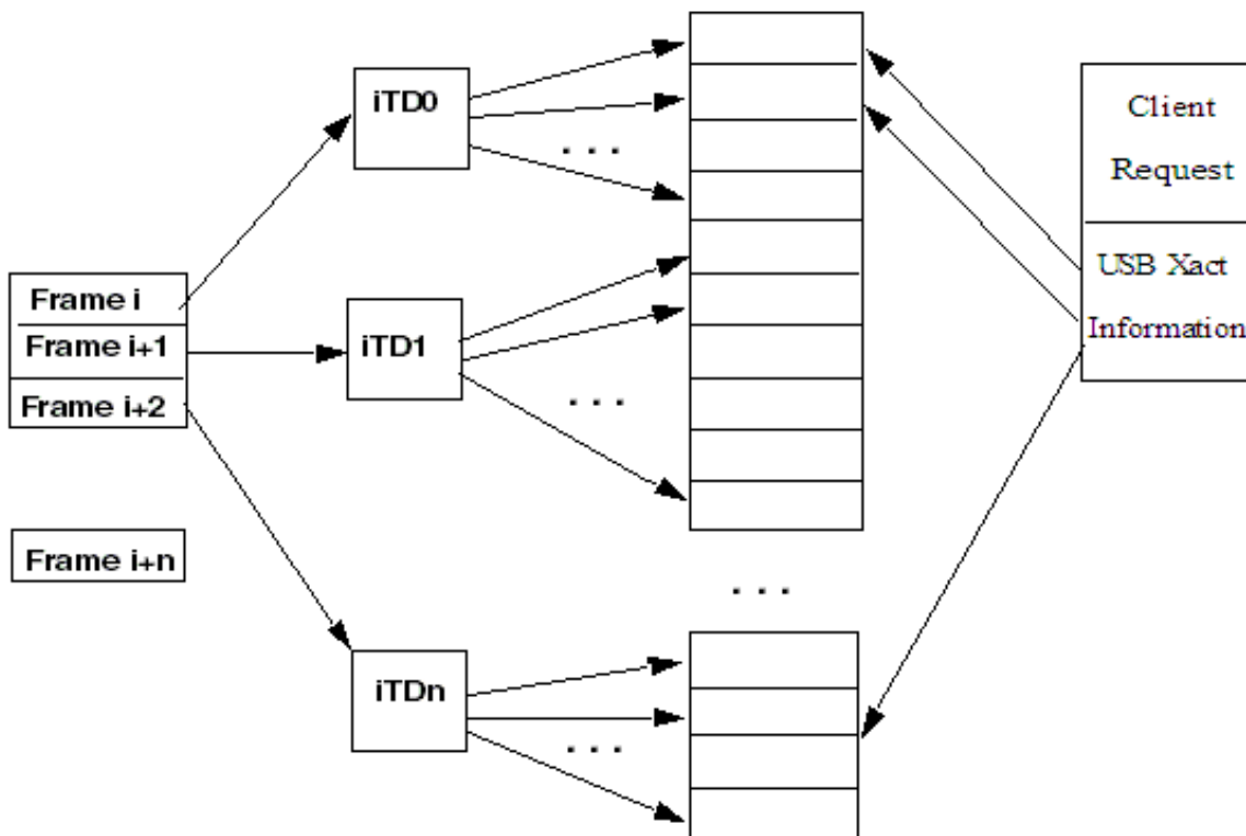
Figure 43-150. Example Association of iTDs to Client Request Buffer
