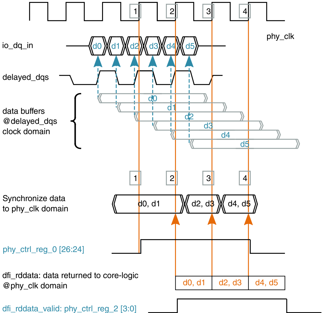
Figure 34-201. Synchronize Read Data
