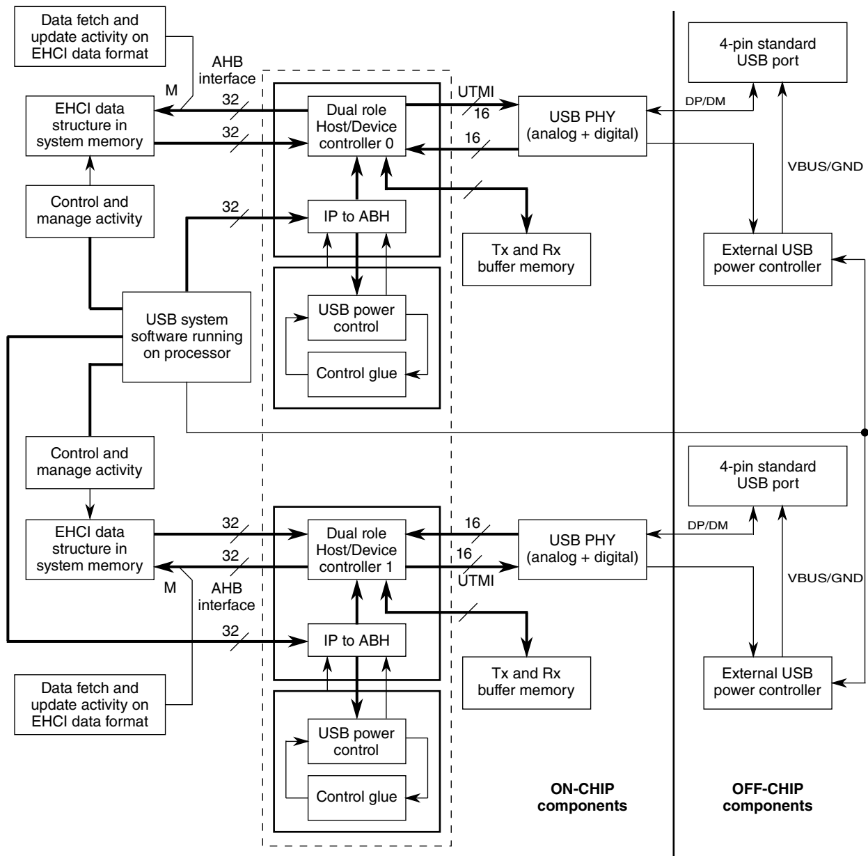
Figure 43-1. USB block diagram
