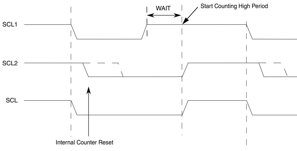
Figure 48-40. I 2 C bus clock synchronization
