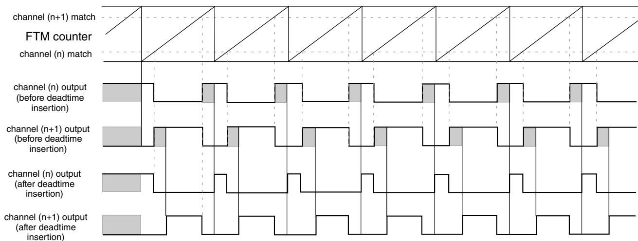
Figure 39-270. Deadtime insertion with ELSnB:ELSnA = X:1 , POL(n) = 0 , and POL(n+1) = 0
