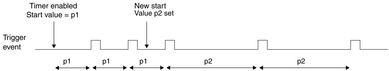
Figure 40-43. Dynamically setting a new load value
