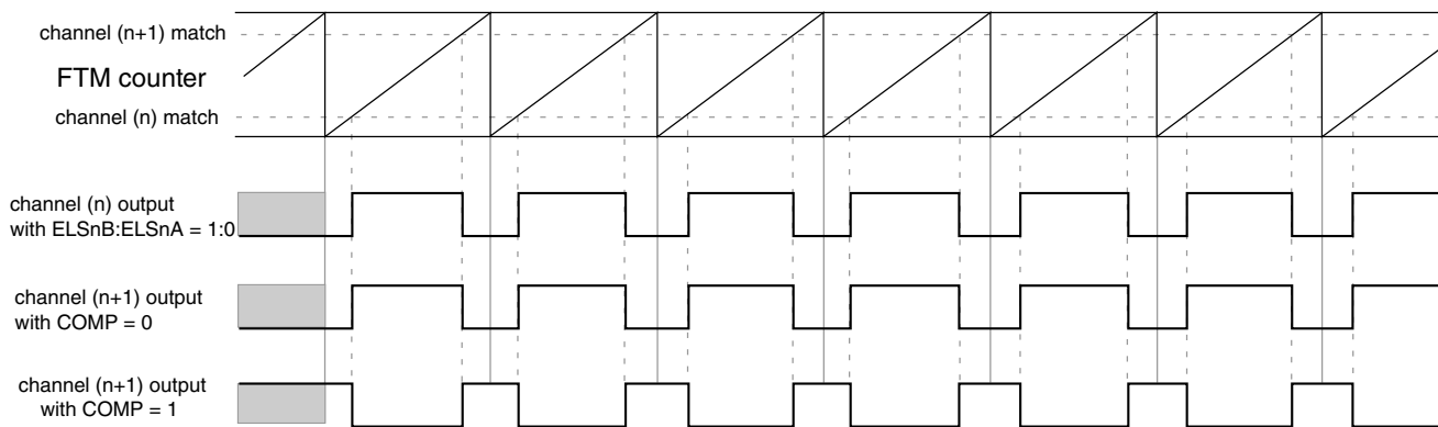
Figure 39-244. Channel (n+1) output in Complementary mode with (ELSnB:ELSnA = 1:0)
