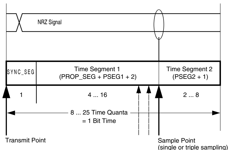
Figure 46-273. Segments within the bit time
