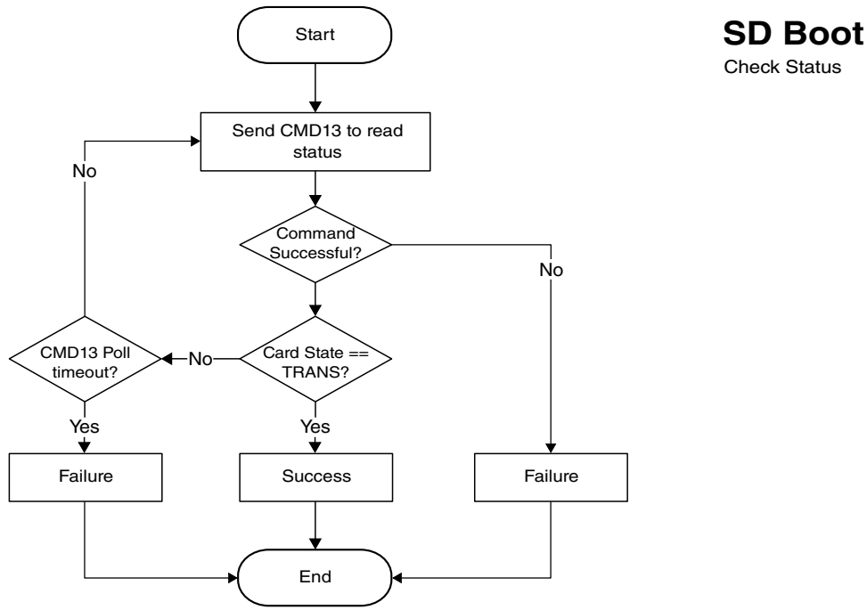
Figure 19-12. Expansion Device Boot Flow (5/7)
