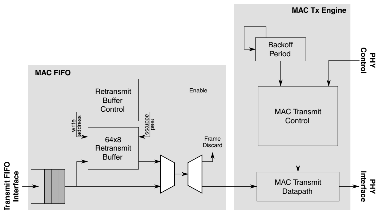
Figure 42-307. Packet re-transmit overview
