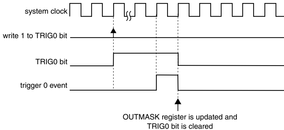
Figure 39-257. OUTMASK synchronization with (SYNCMODE = 0), (HWTRIGMODE = 0), (SYNCHOM = 1), (PWMSYNC = 0), and a hardware trigger was used
