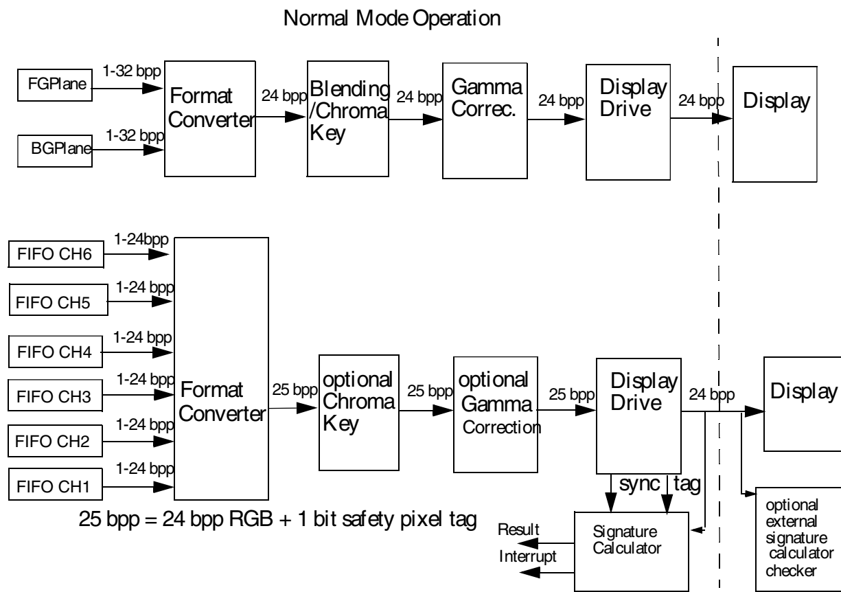
Figure 55-1945. Safety Mode Block Diagram
