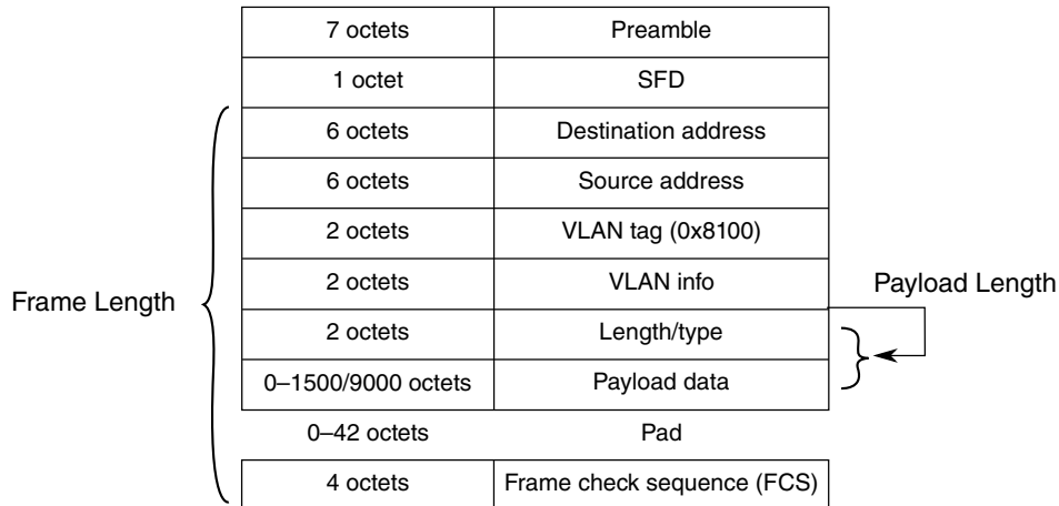
Figure 42-303. VLAN-tagged MAC frame format overview
