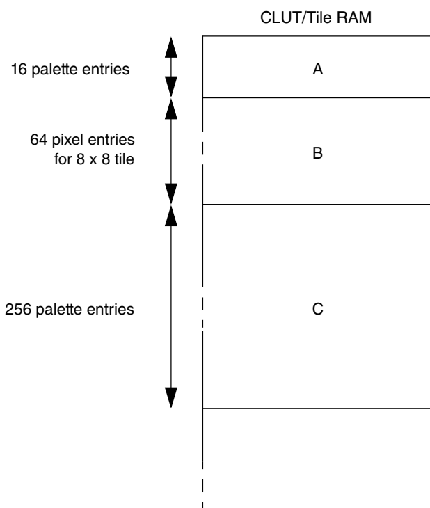
Figure 55-1941. An example of use for the CLUT/Tile RAM
