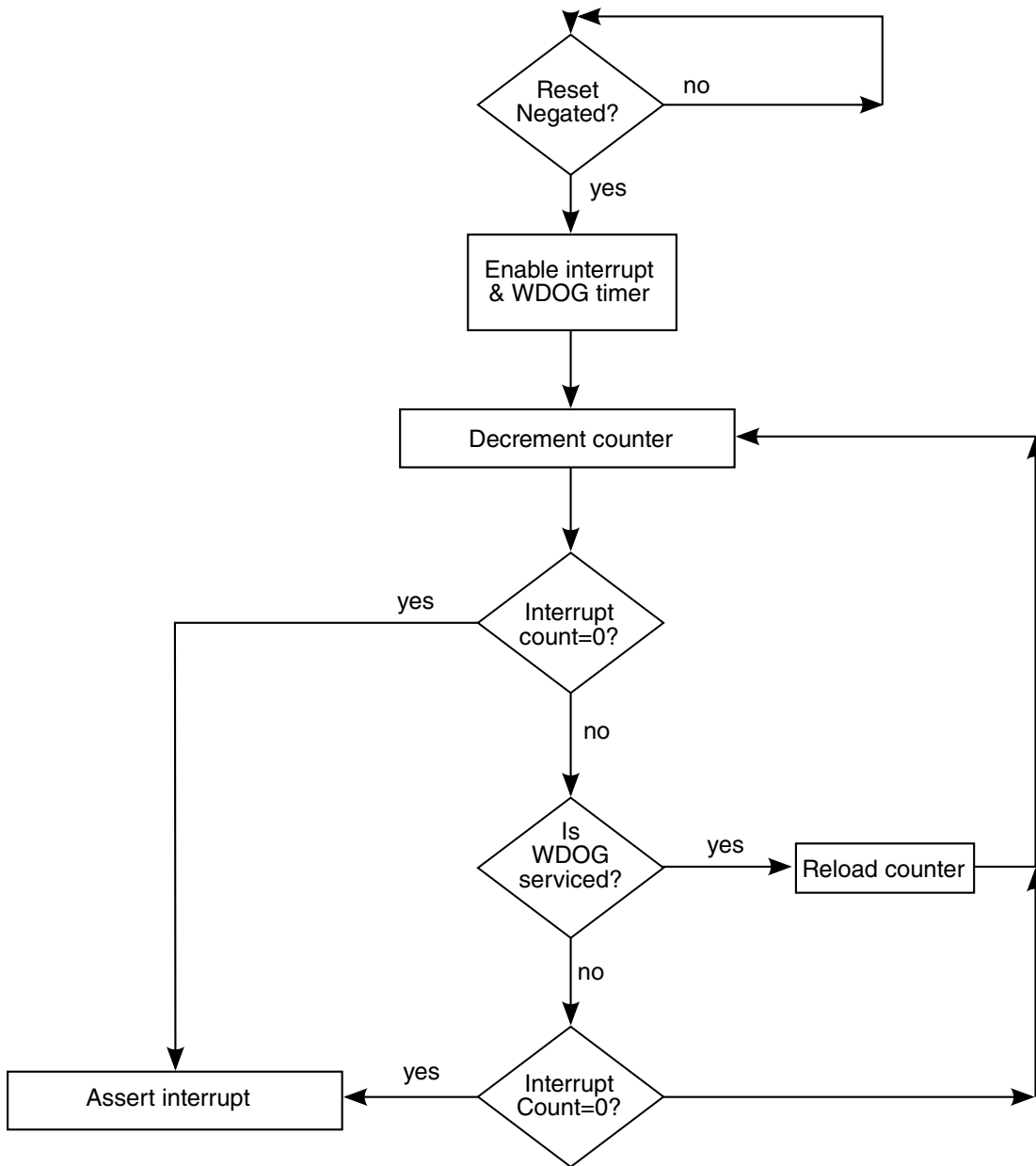
Figure 26-6. Interrupt Generation Flow Diagram
