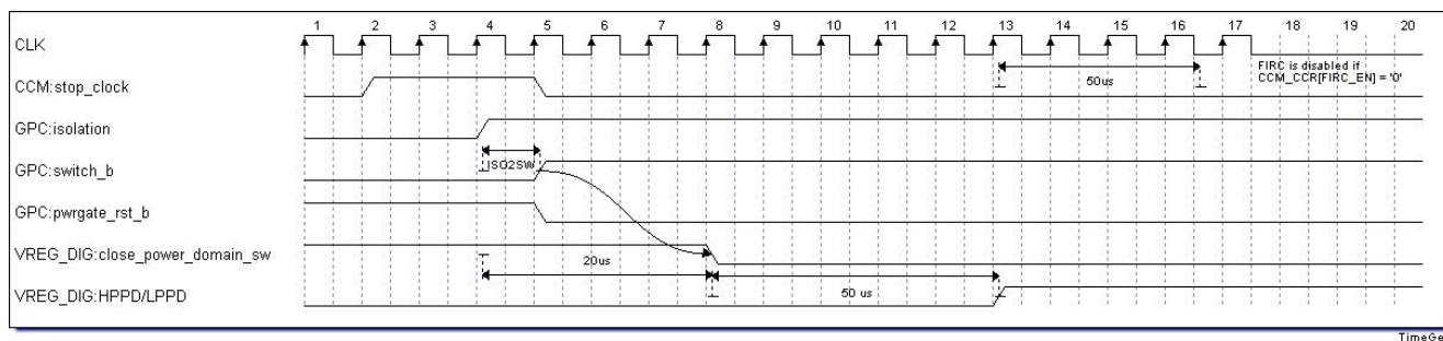
Figure 15-7. Power-Down Sequence Timing Diagram
