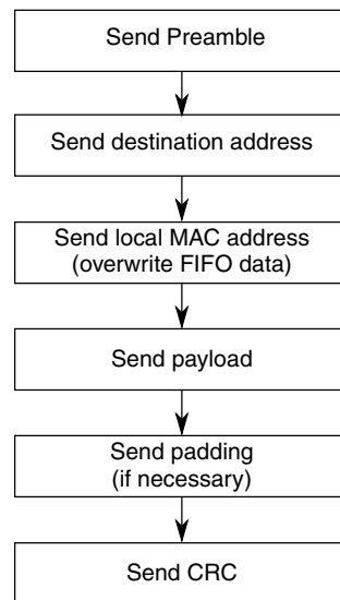
Figure 42-306. Frame transmit overview
