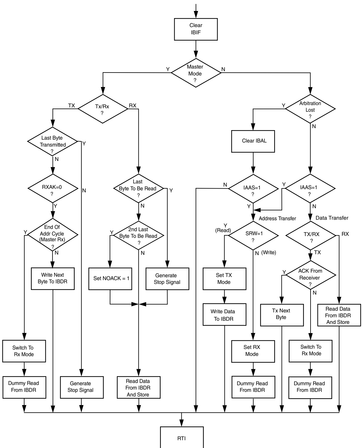
Figure 48-48. Recommended I 2 C interrupt service routine flowchart
