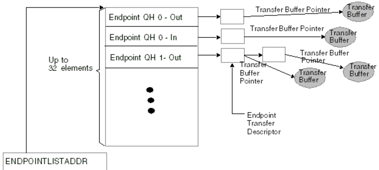
Figure 43-167. End Point Queue Head Diagram
