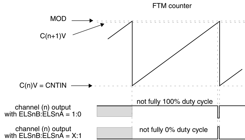
Figure 39-233. Channel (n) output if (C(n)V = CNTIN) and (CNTIN < C(n+1)V < MOD) and (C(n+1)V is Almost Equal to MOD )
