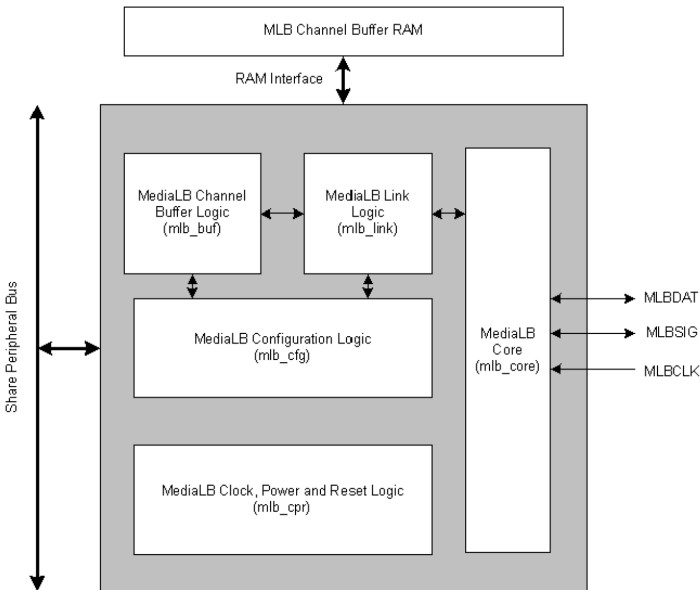
Figure 45-1. Block Diagram
