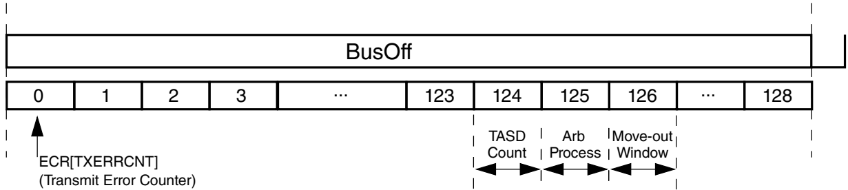
Figure 46-276. Arbitration at the end of bus off and move-out time windows
