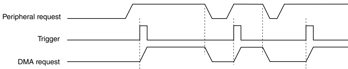
Figure 22-88. DMAMUX channel triggering: normal operation
