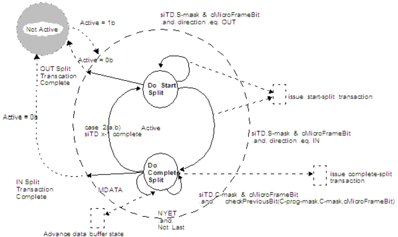
Figure 43-164. Split Transaction State Machine for Isochronous
