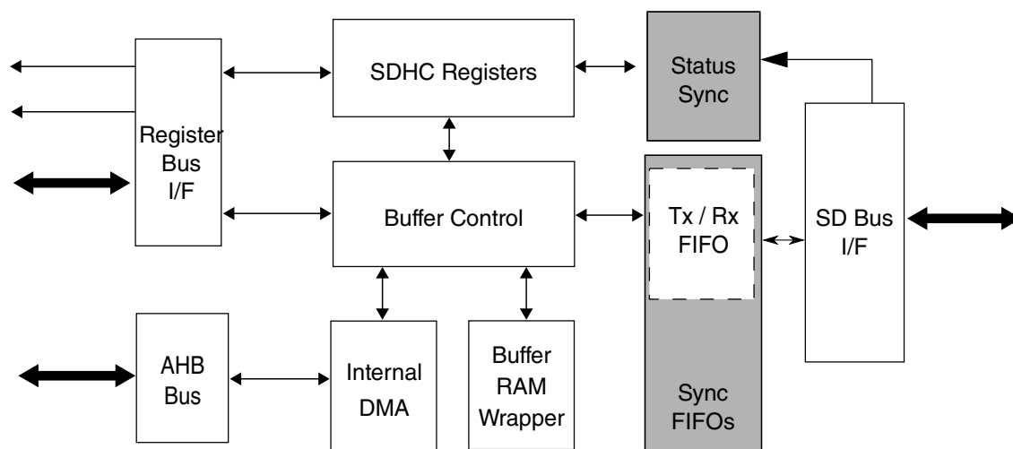
Figure 50-75. SDHC buffer scheme
