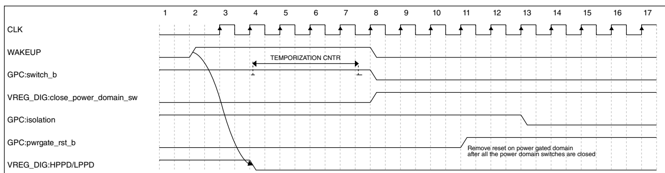
Figure 15-8. Power-Up Sequence Timing Diagram
