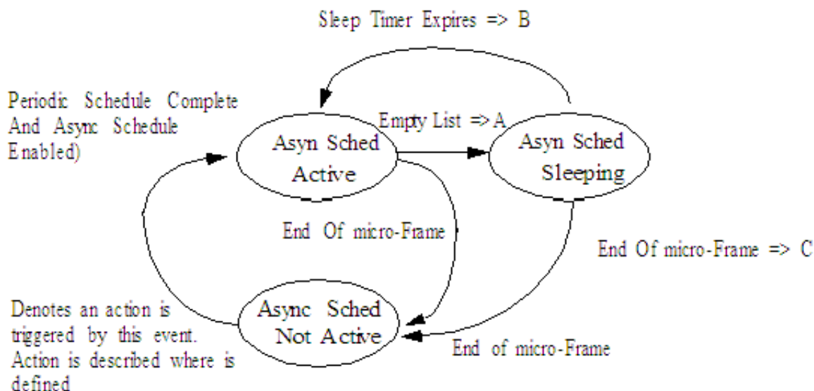
Figure 43-153. Example State Machine for Managing Asynchronous Schedule Traversal
