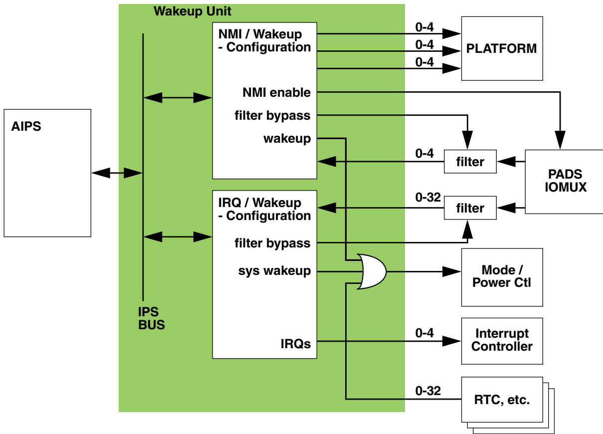
Figure 28-1. WKPU and connected system components
