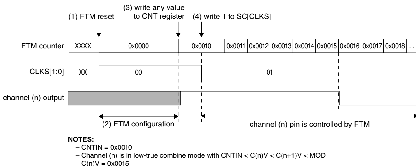
Figure 39-300. FTM behavior after reset when the channel (n) is in Combine mode
