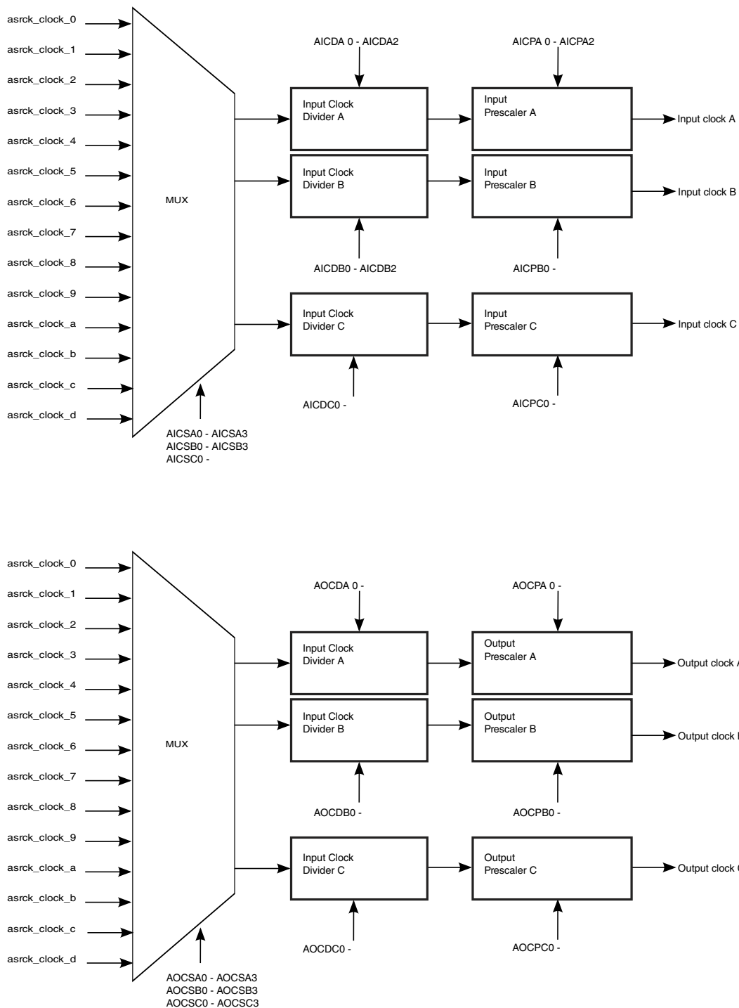
Figure 53-46. Clock Source Selector & Divider
