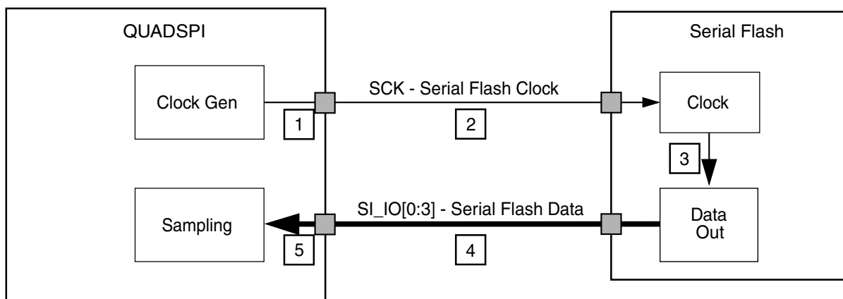
Figure 30-420. Serial Flash Sampling Clock Overview
