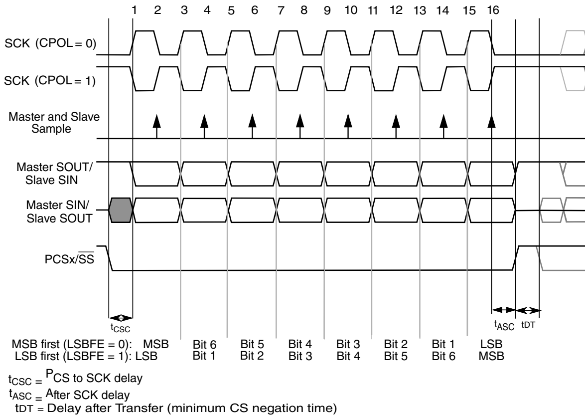
Figure 47-127. Module transfer timing diagram (MTFE=0, CPHA=1, FMSZ=8)
