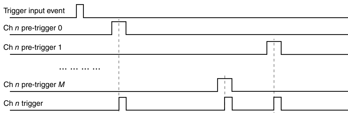
Figure 38-24. Pre-trigger and trigger outputs
