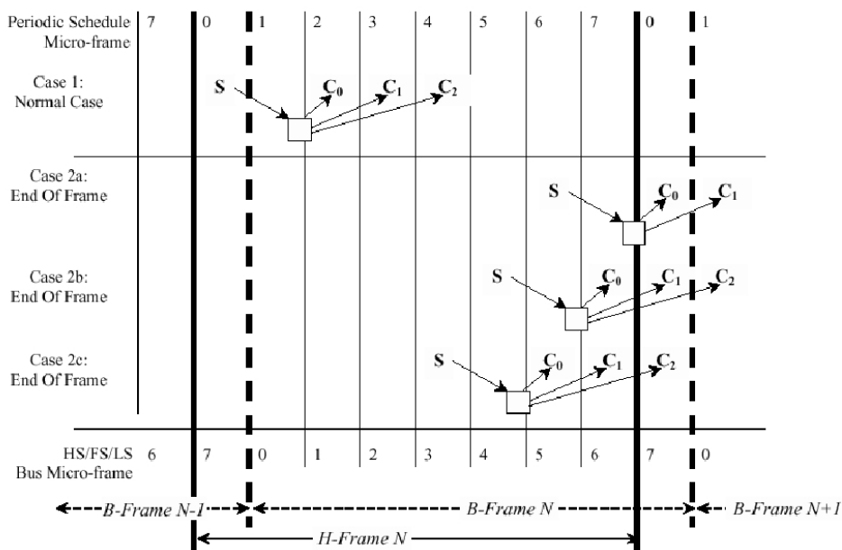
Figure 43-158. Split Transaction, Interrupt Scheduling Boundary Conditions
