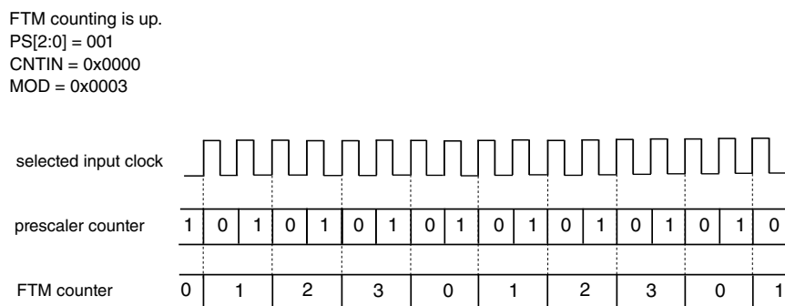
Figure 39-208. Example of the prescaler counter
