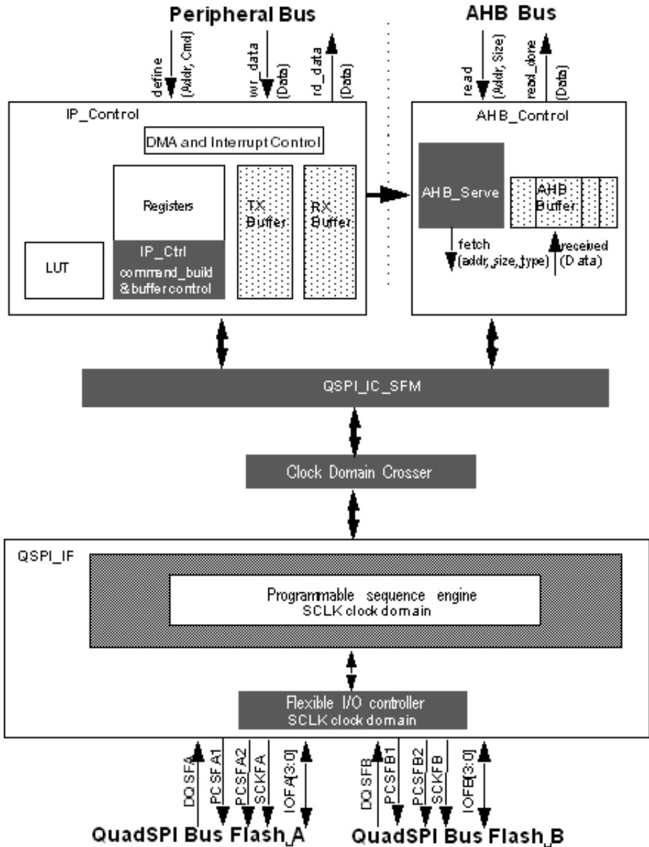
Figure 30-1. QuadSPI Block Diagram
