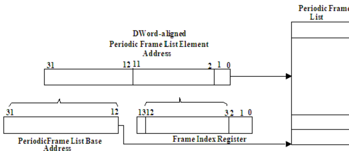
Figure 43-144. Derivation of Pointer into Frame List Array
