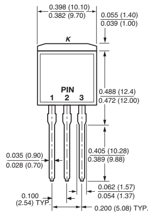
TO-262AA
