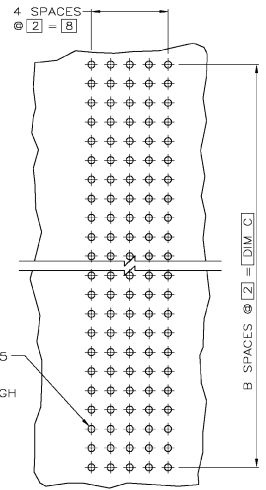
RECOMMENDED CIRCUIT PATTERN (COMPONENT SIDE)
