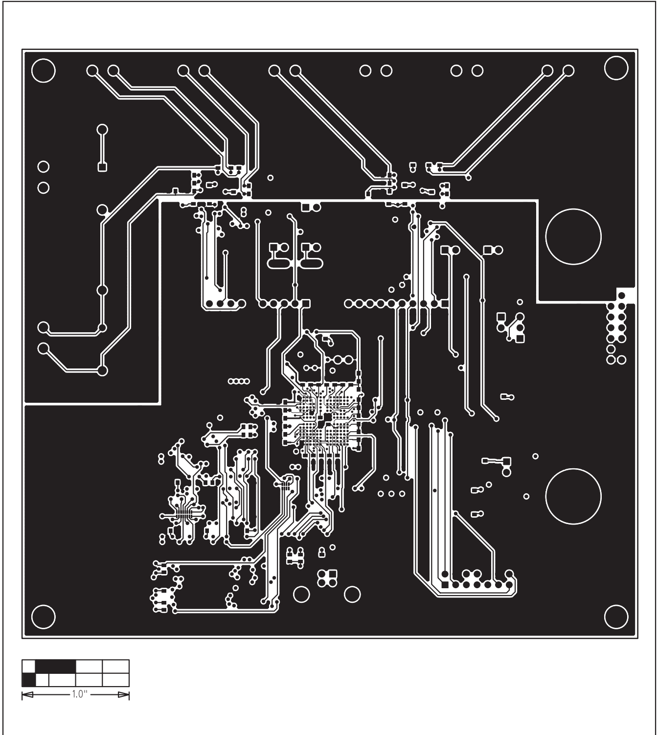
Figure 9. MAX11040 EV Kit PCB Layout—Bottom Side
