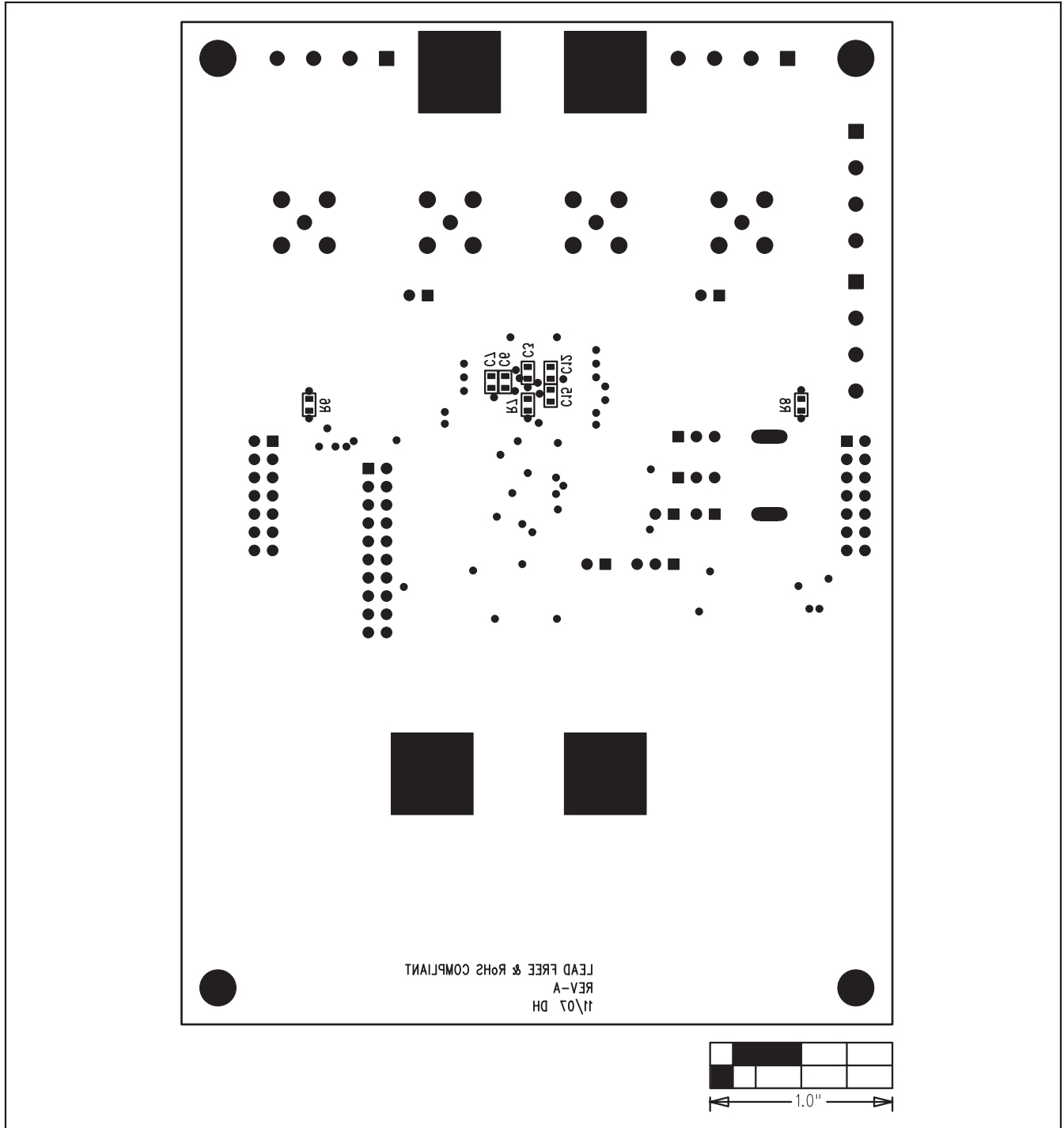
Figure 17. MAX11040 Daughterboard Component Placement Guide—Bottom
