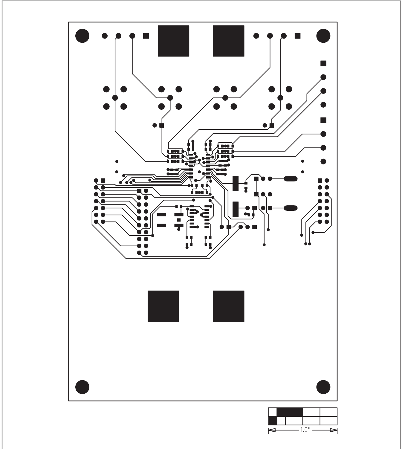
Figure 13. MAX11040 Daughterboard PCB Layout—Component Side
