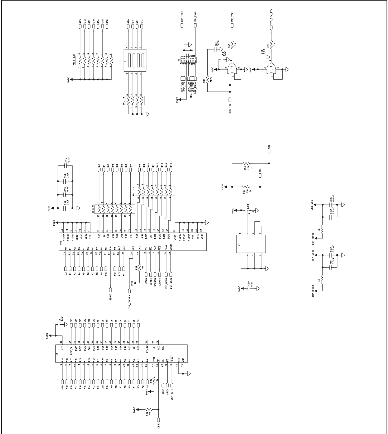
Figure 2c. MAX11040 EV Kit Schematic (Sheet 3 of 4)
