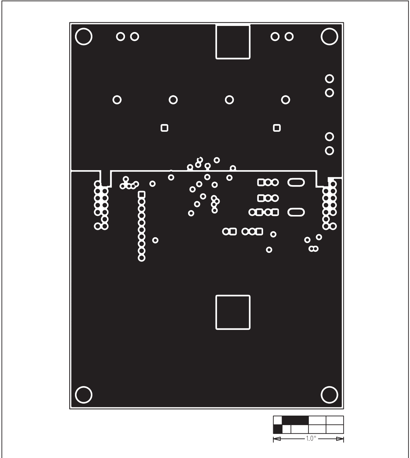
Figure 14. MAX11040 Daughterboard PCB Layout—Layer 2
