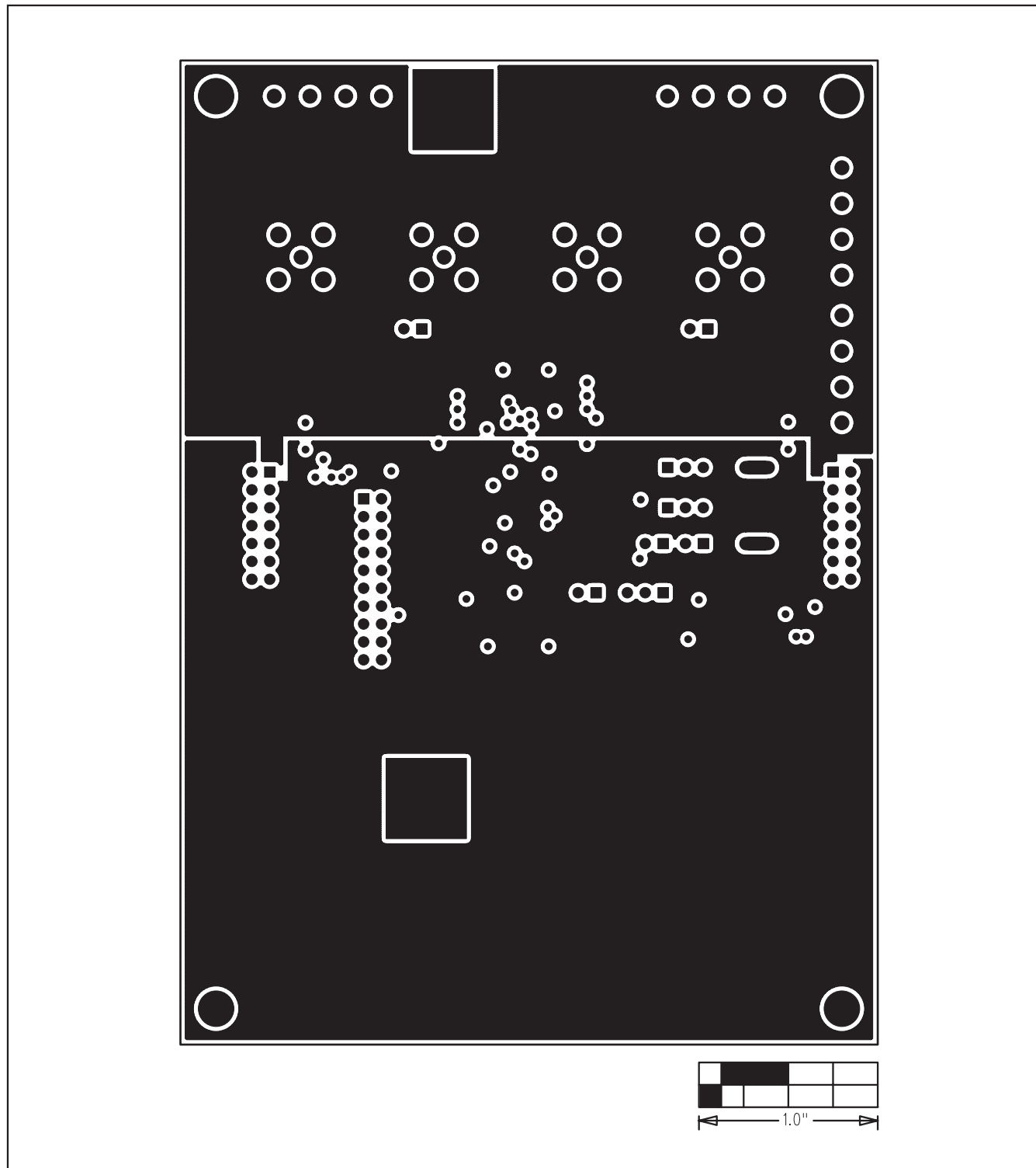
Figure 15. MAX11040 Daughterboard PCB Layout—Layer 3
