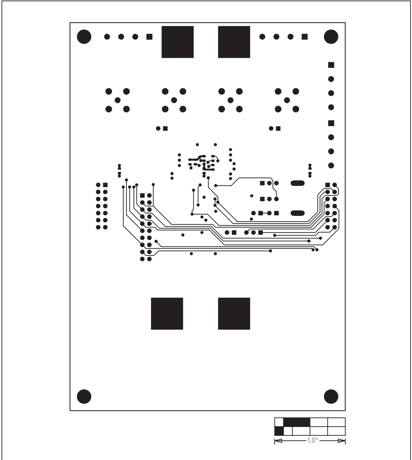
Figure 16. MAX11040 Daughterboard PCB Layout—Bottom
