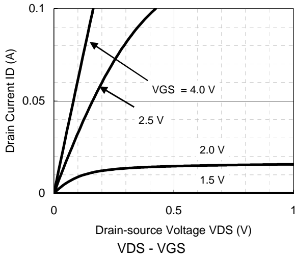
ID - VDS
